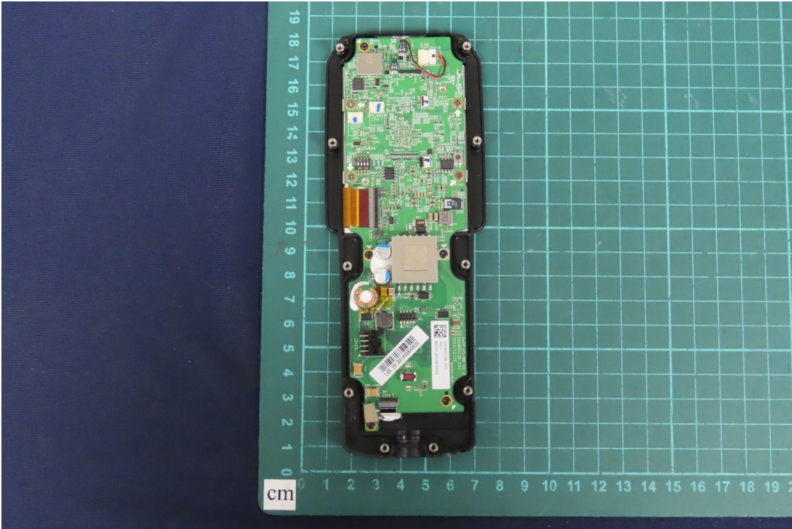
(27) EUT Photo
