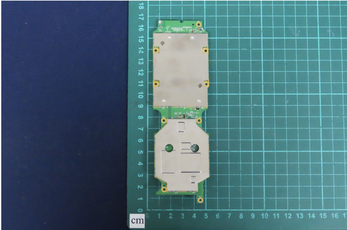
(22) EUT Photo
