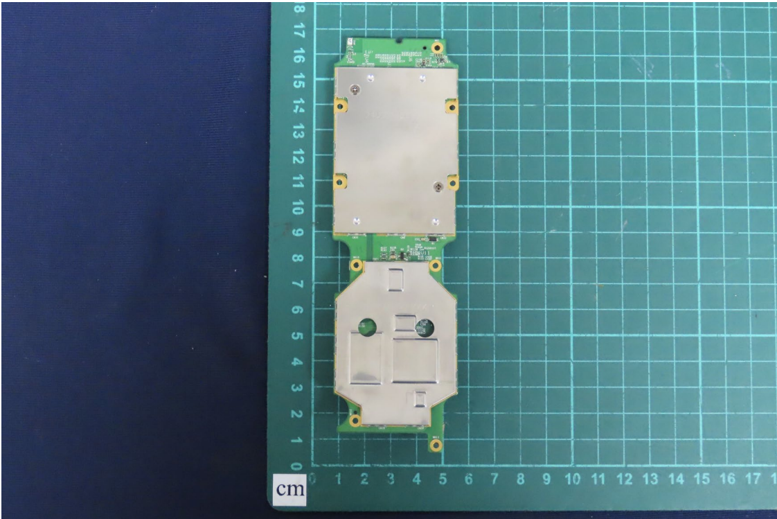
(34) EUT Photo
