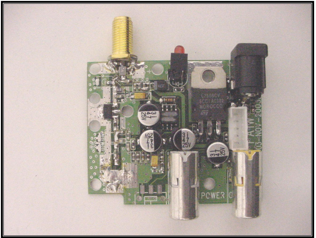
PHOTOGRAPH 12: TOP OF PCB1
