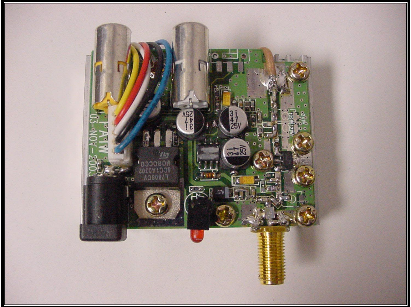
PHOTOGRAPH 8: TOP WITH CASE REMOVED
