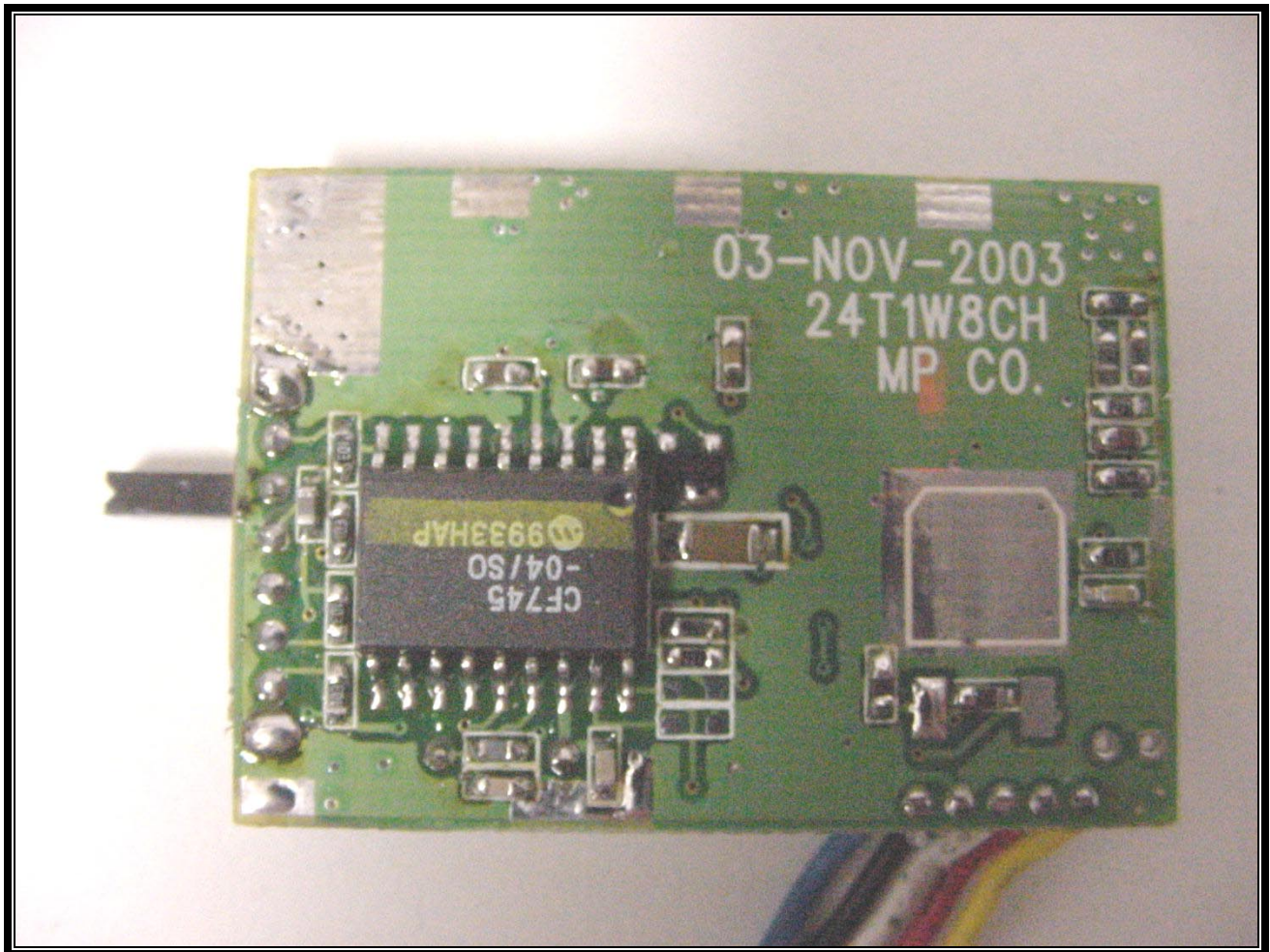
PHOTOGRAPH 15: BOTTOM OF PCB2
