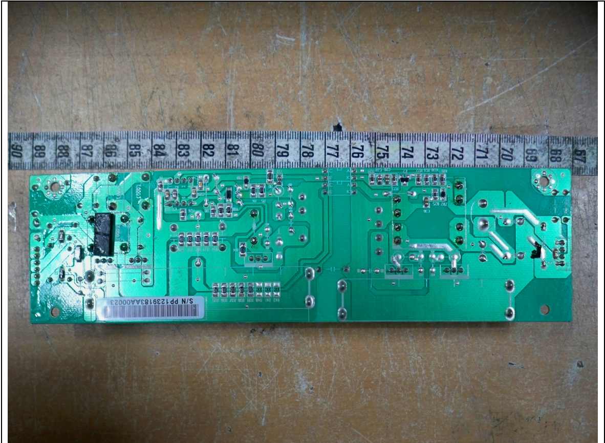
SMPS – Rear
