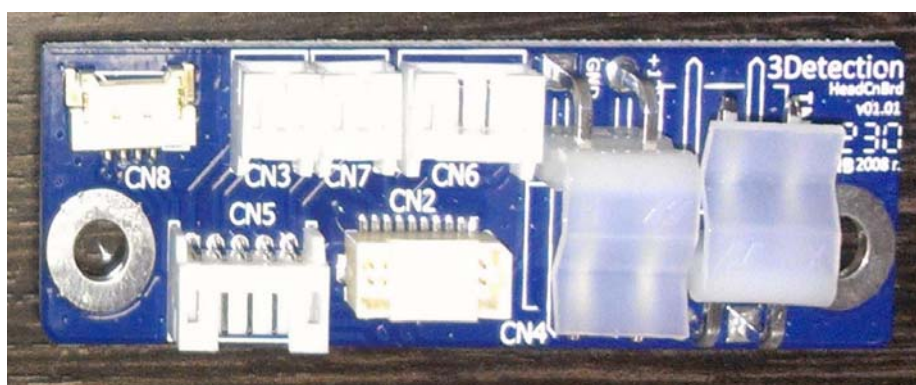
Socket Adapter 2-2
