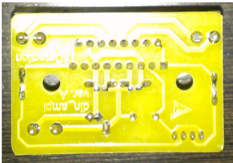
Audio Amplifier 1
