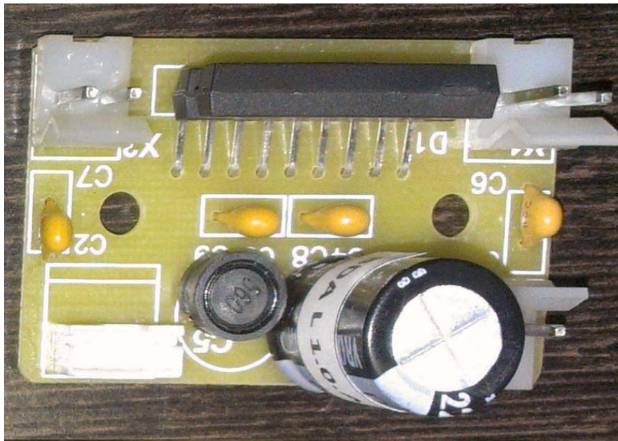
Audio Amplifier 2
