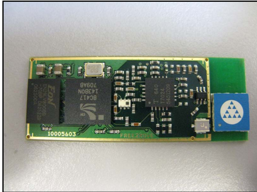
Photograph 13: Bluetooth Radio Top
