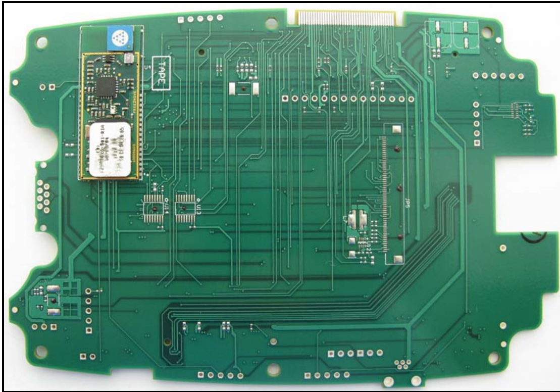
Photograph 9: Bottom View
