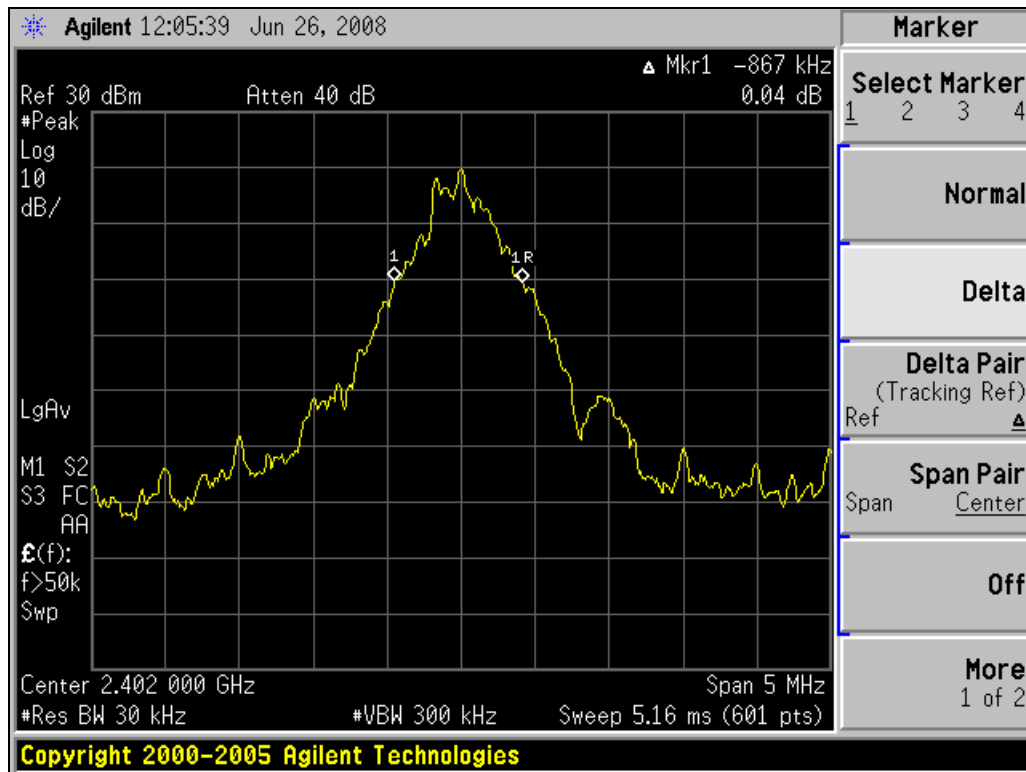
Plot 6-1: 20 dB Bandwidth 2402 MHz
