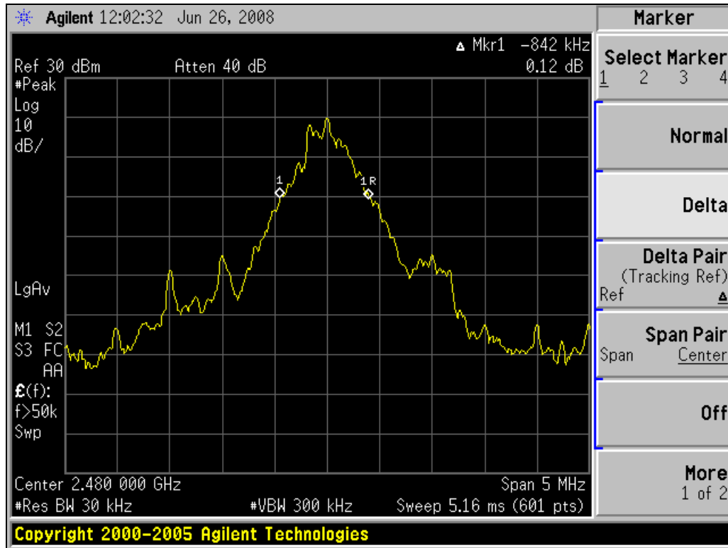
Plot 6-3: 20 dB Bandwidth 2480 MHz
