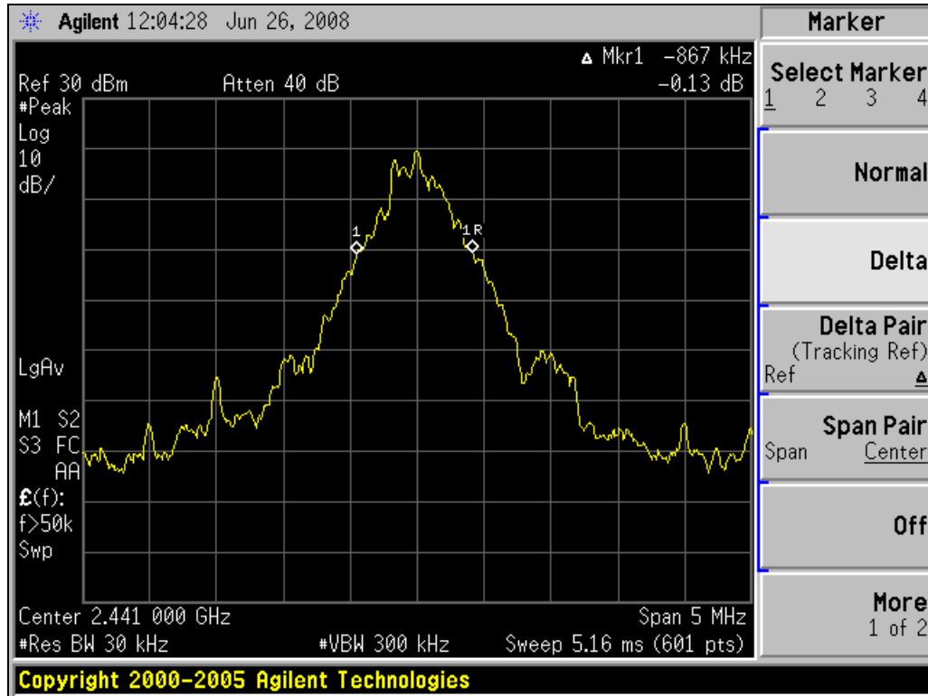
Plot 6-2: 20 dB Bandwidth 2441 MHz
