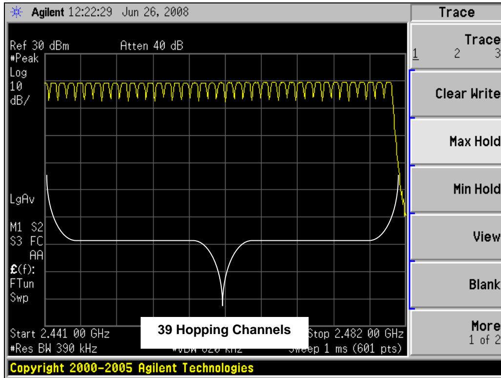
Plot 8-2: Number of Hopping Frequencies
