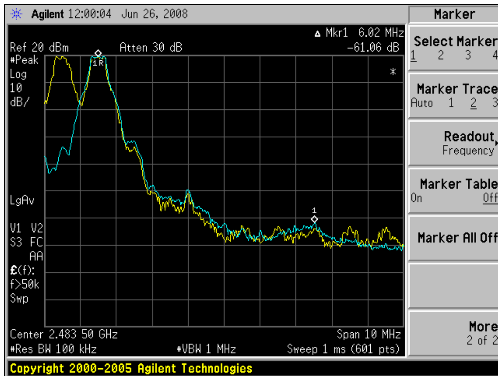
Plot 4-2: Upper Band Edge (Fixed Frequency 2480 MHz in Blue, Hopping in Yellow)
