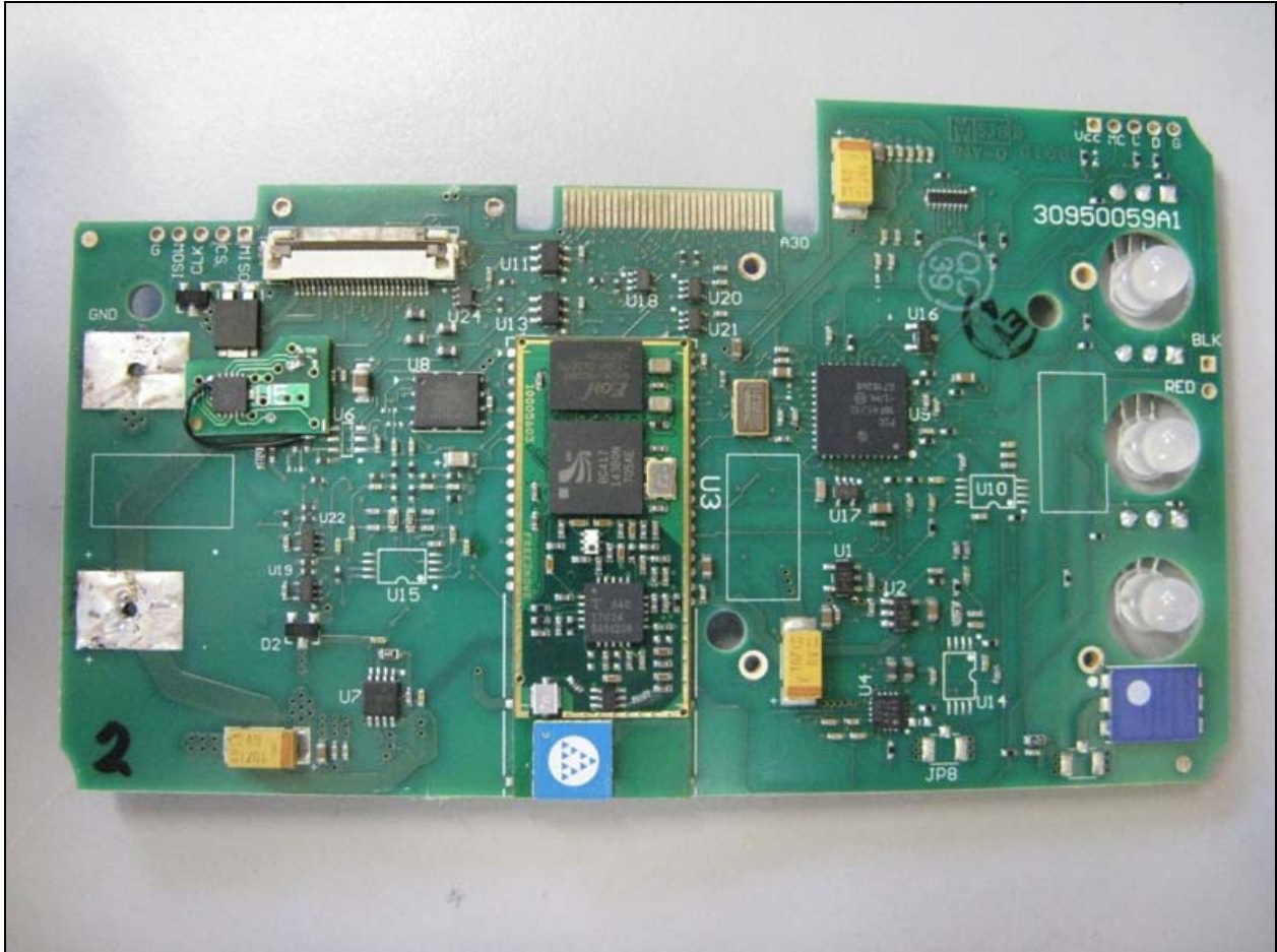
Photograph 17: Comm Board with Bluetooth Module
