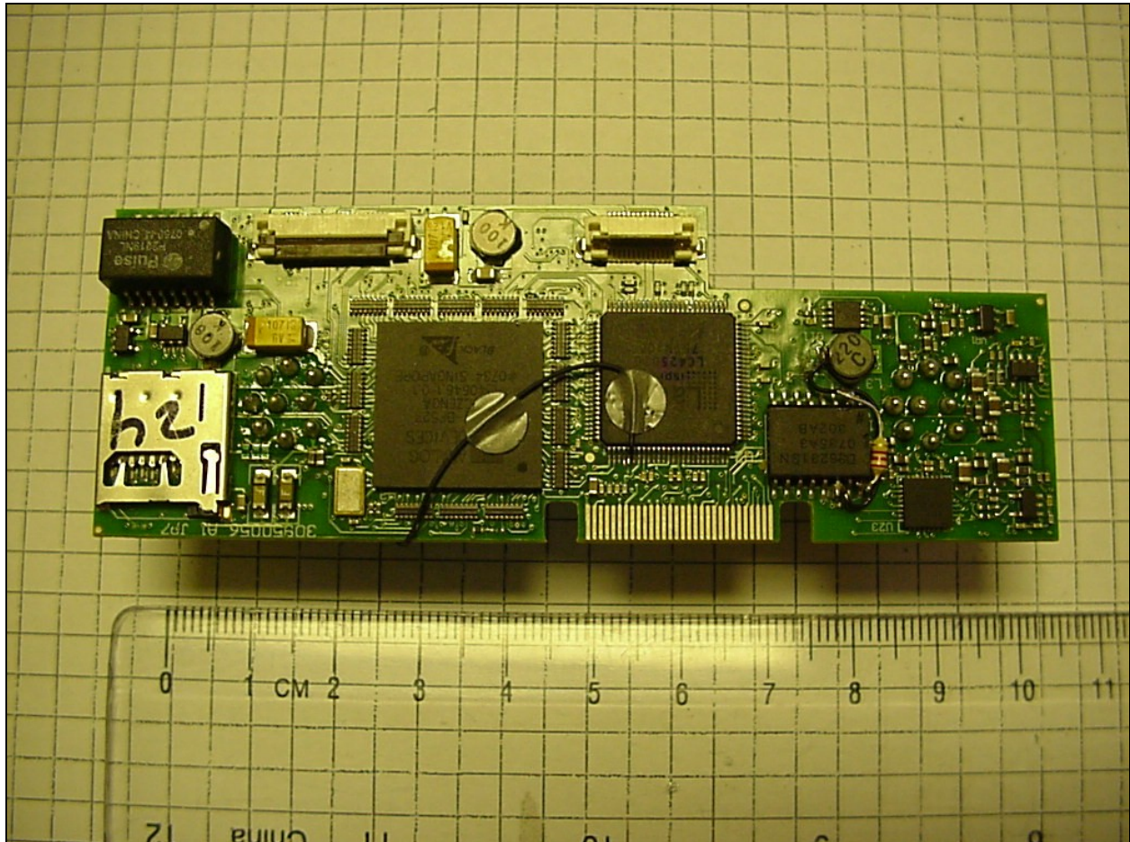
Photograph 13: Digital PCB Inside
