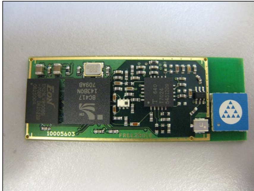
Photograph 18: Bluetooth Radio Top
