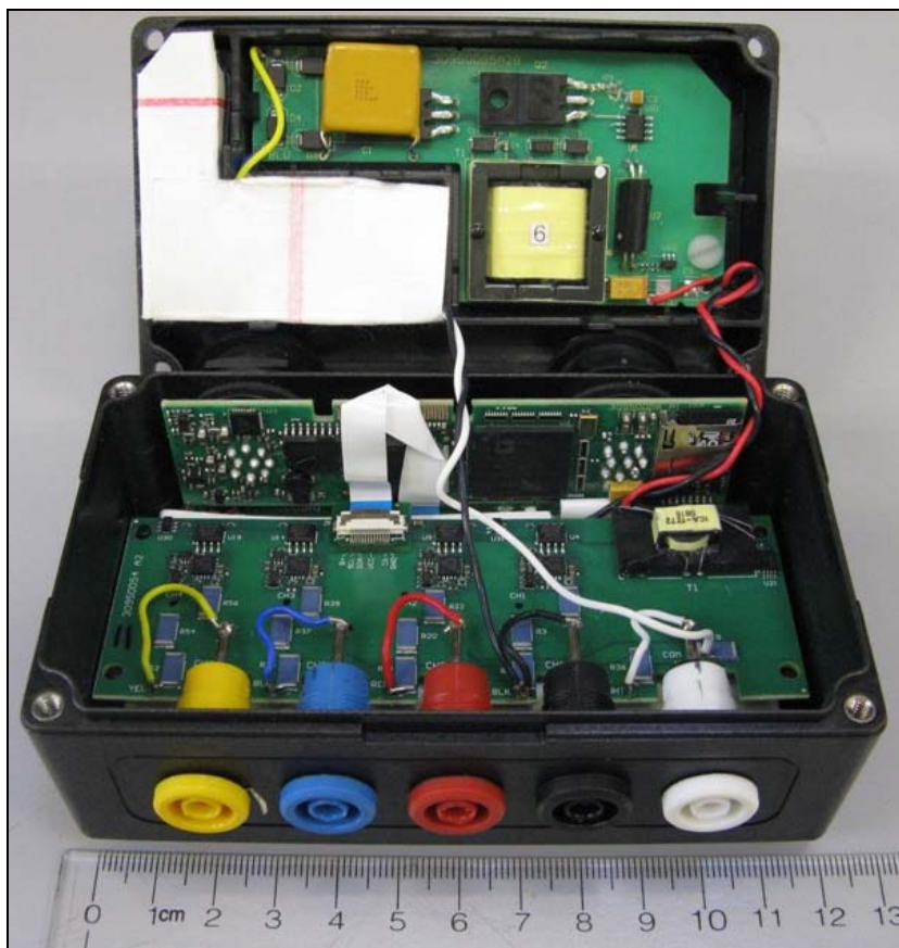
Photograph 10: PCBs Mounted in the Housing
