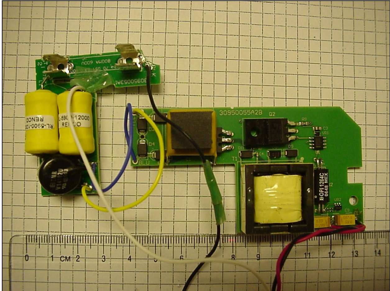
Photograph 16: Power Supply PCBs Top
