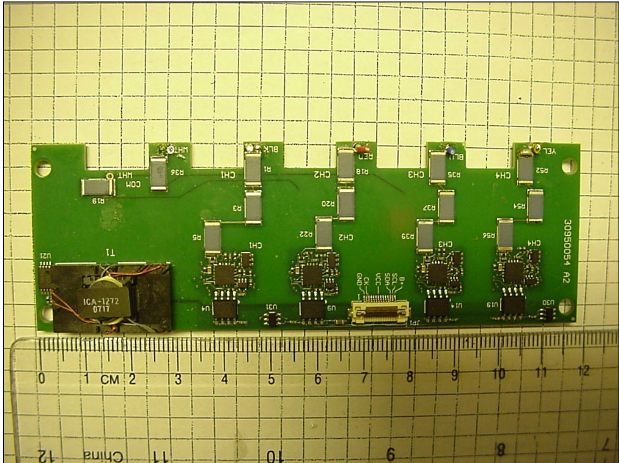
Photograph 12: Digital Isolator PCB Bottom
