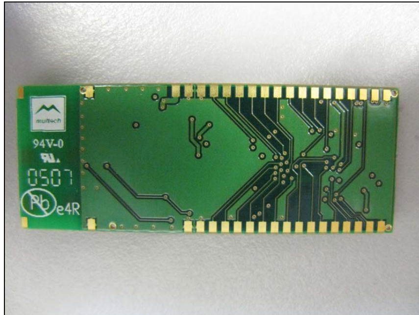
Photograph 19: Bluetooth Radio Bottom
