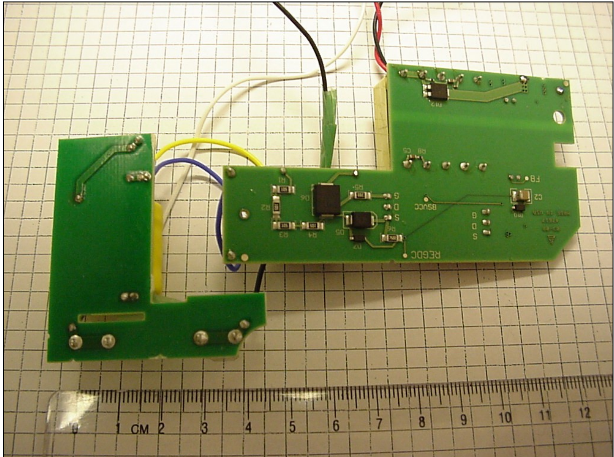
Photograph 15: Power Supply PCBs Bottom
