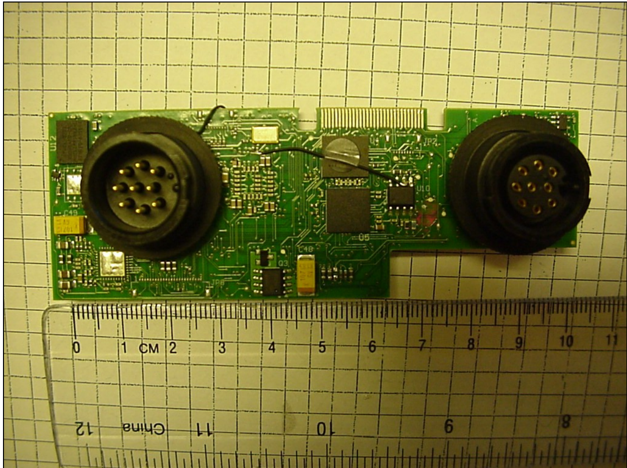
Photograph 14: Digital PCB Outside
