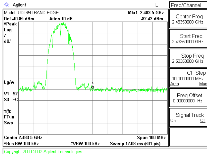
Plot A-11. 36 Mbps Occupied Band Edge Plot – Ch. 11
