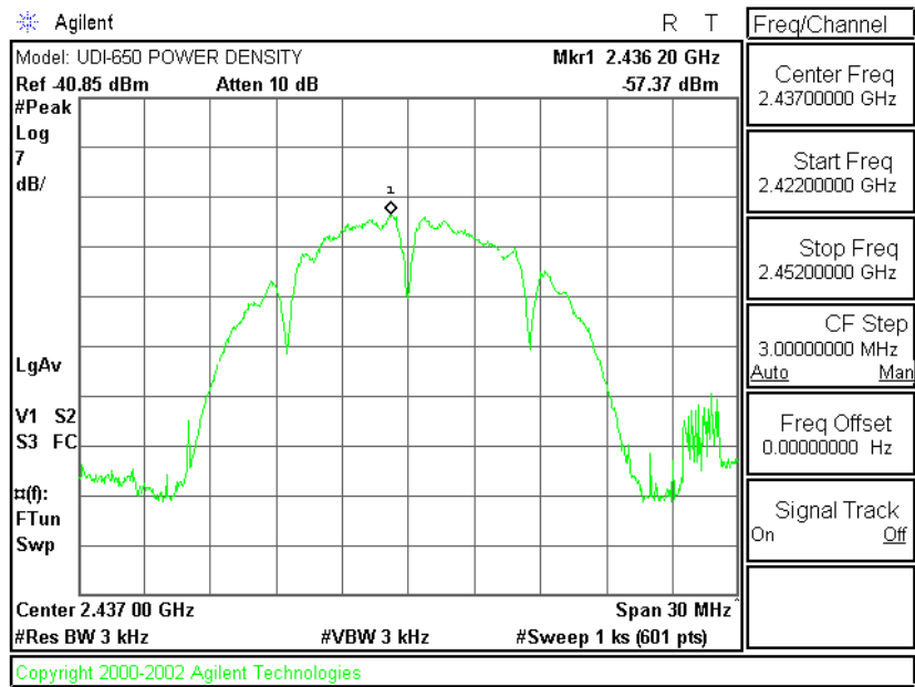
Plot A-8. Max. Power Density Plot – Ch. 6
