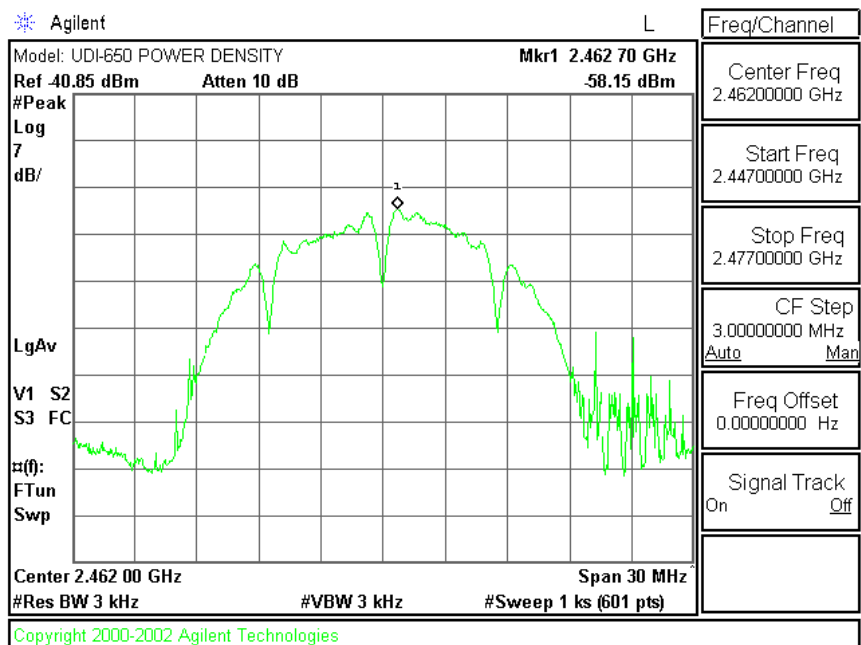
Plot A-9. Max. Power Density Plot – Ch. 11
