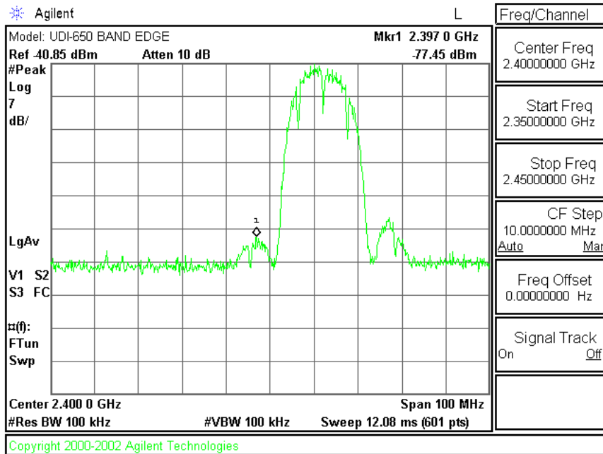
Plot A-10. 36 Mbps Occupied Band Edge Plot – Ch. 01
