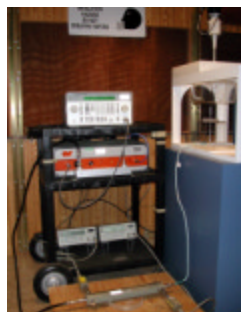
Figure A.0 Dipole Validation Test Setup
