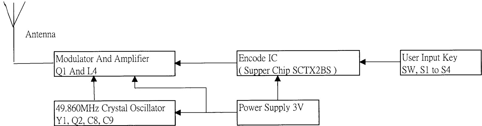
The Block Diagram Of Transmitting Circuit For 49.860MHz
