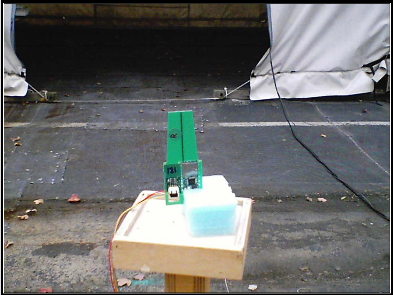
Photograph 1: Radiated Emissions Testing Front View
