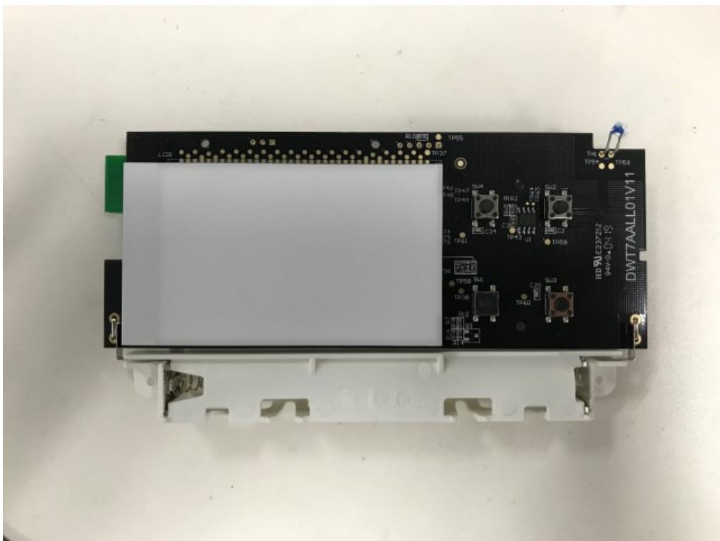
Internal View (Model: WRT2-TX)
