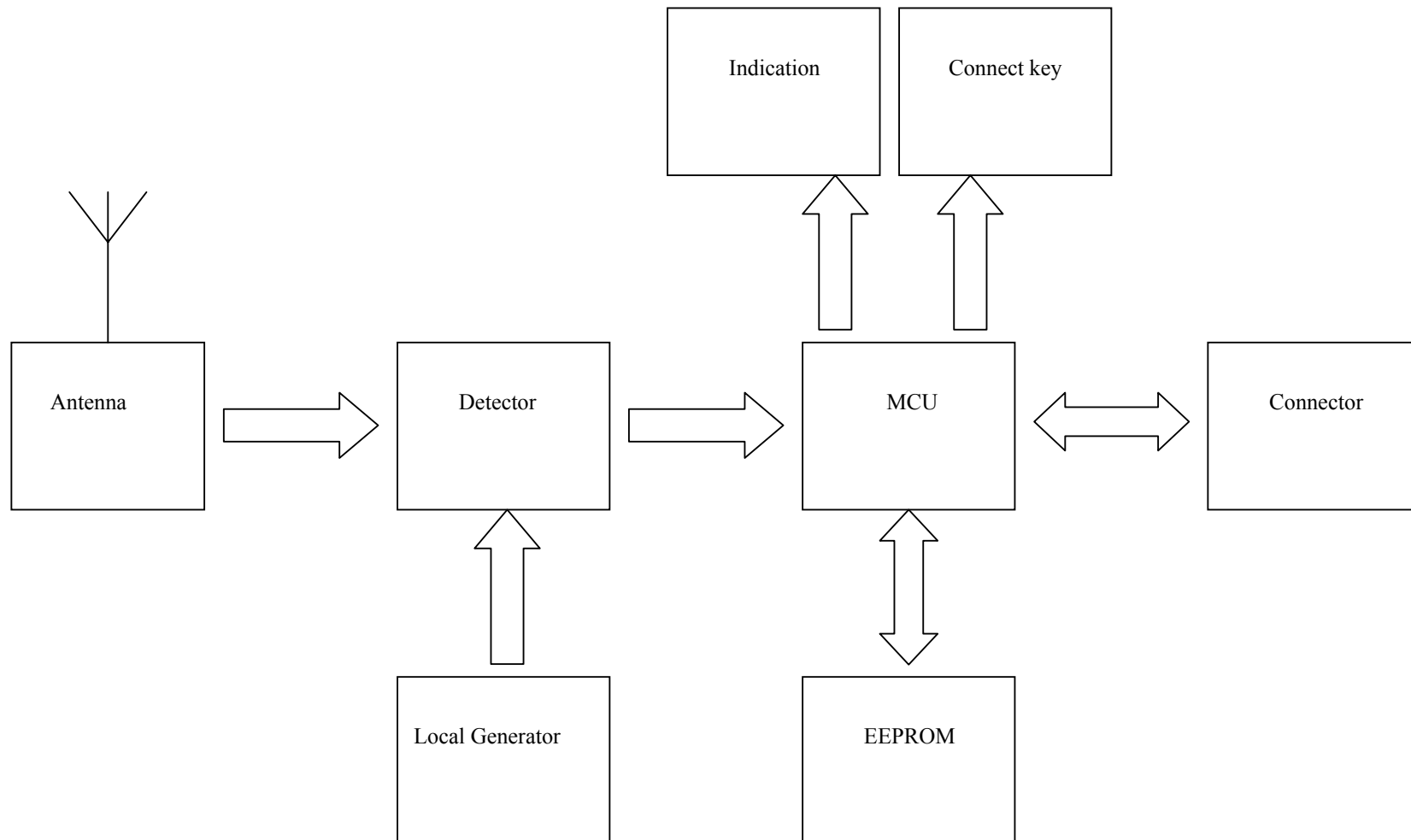
DS-2068 RX Block Diagram
