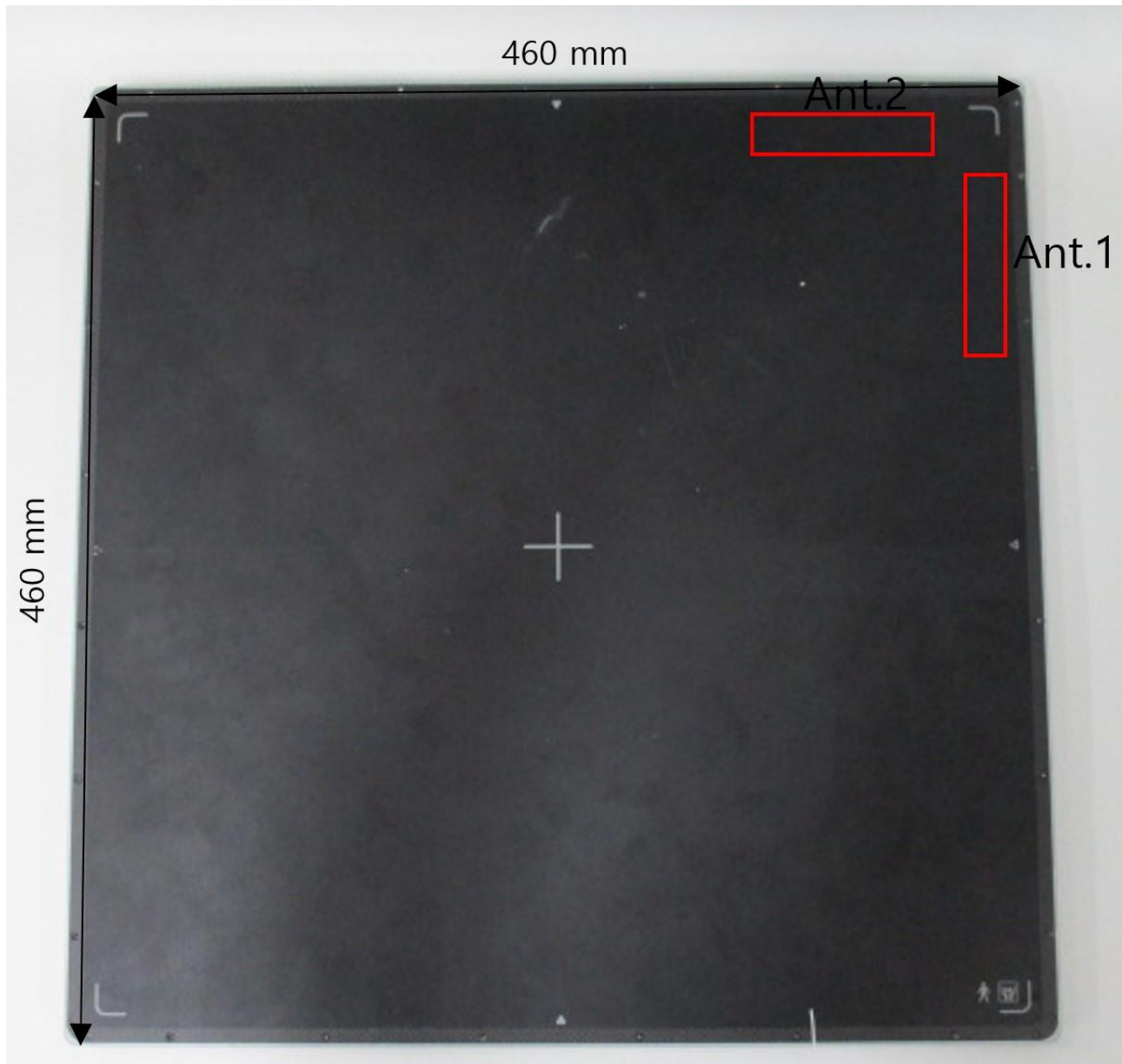
Figure E-2 Antenna Location (Front Side View)
