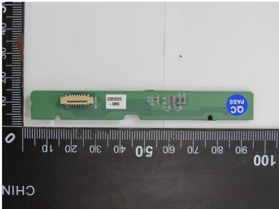
Front View of LCD & Switch Board
