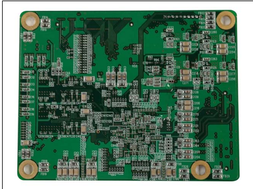
Embedded board(Bottom)
