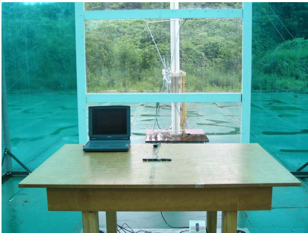
Radiation Test (less than 1GHz)
