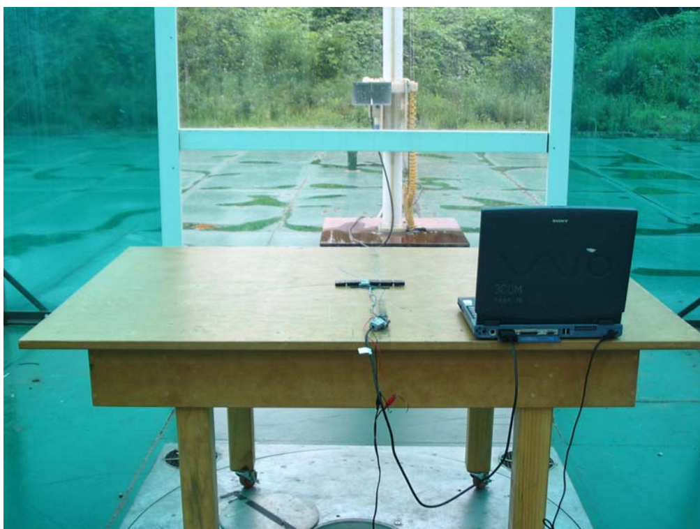
Radiation Test (More than 1GHz)
