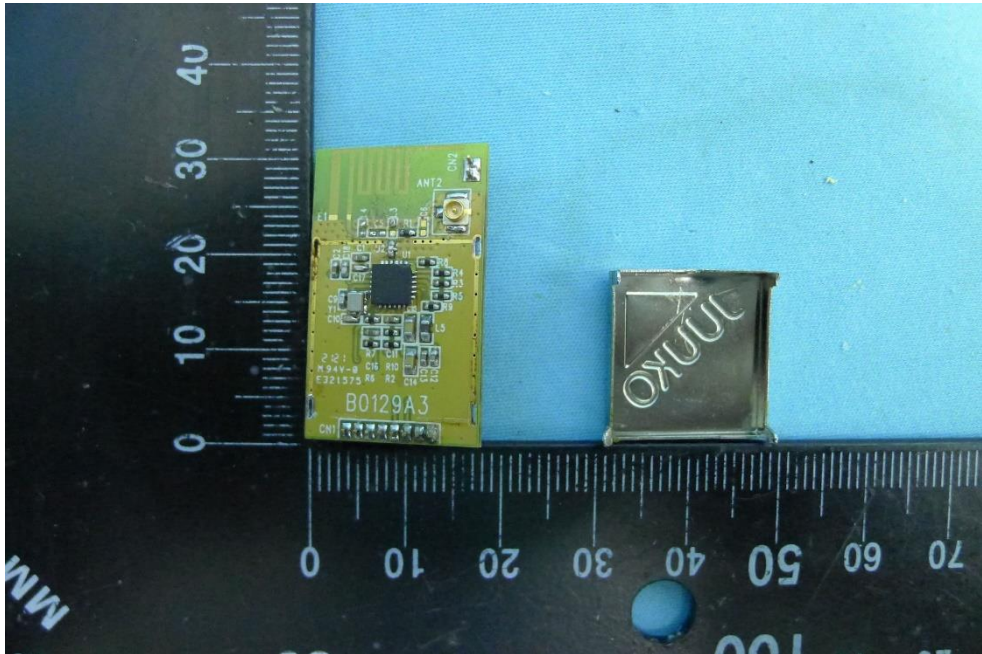
(6) EUT Photo( for External Antenna)
