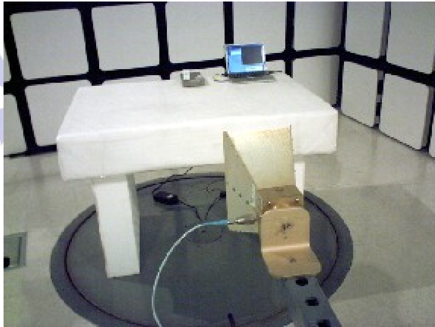
Test Configuration 1. 960 MHz to 40 GHz
