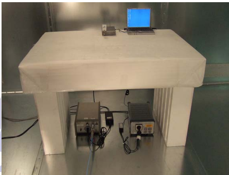
Test Configuration 4 AC mains line-conducted
