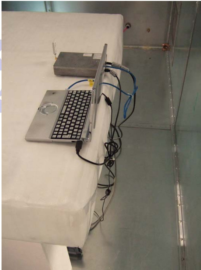
Test Configuration 3 AC mains line-conducted
