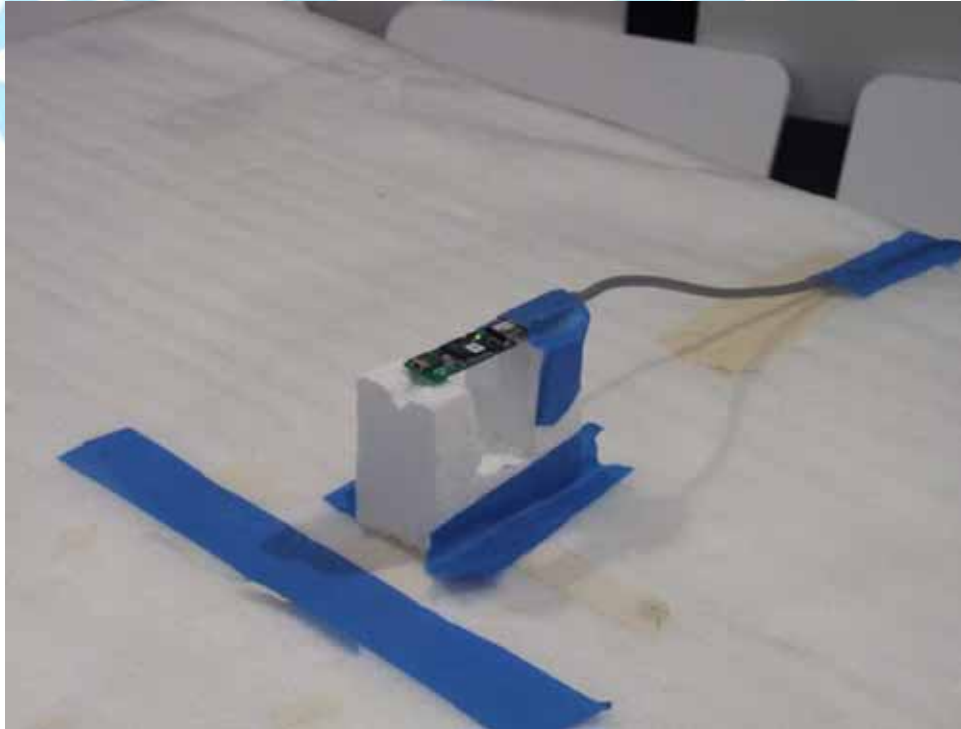
Test Configuration 1: The worst case EUT orthogonal position EUT setting
