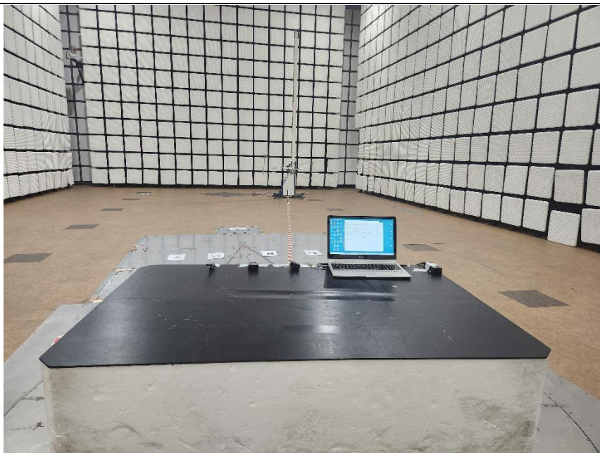
[Rear view of Radiated Emission (30 MHz ~ 1 000 MHz)]
