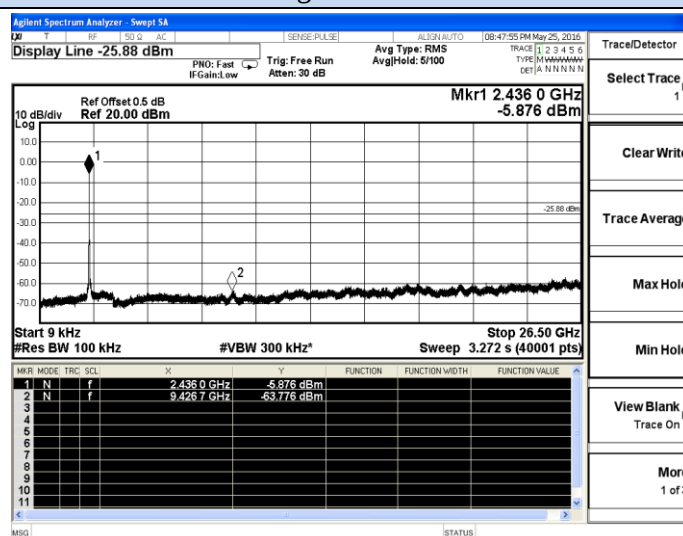
802.11g-Middle channel
