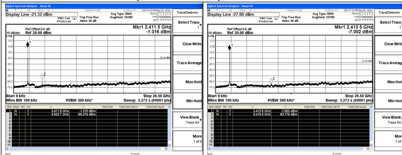
802.11b-Low channel
