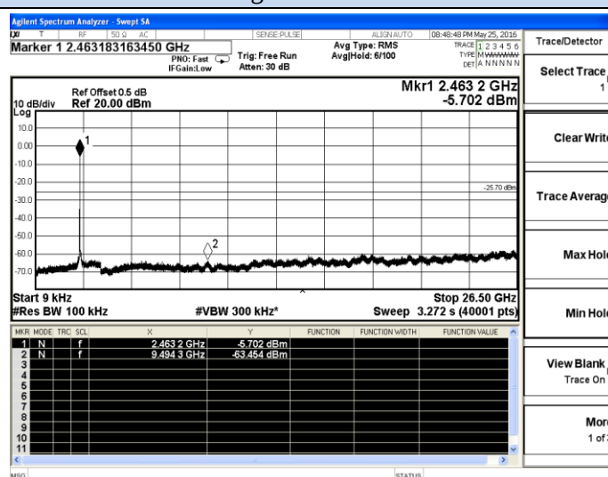
802.11g-High channel
