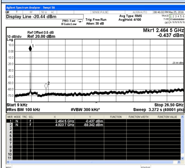
802.11b-High channel
