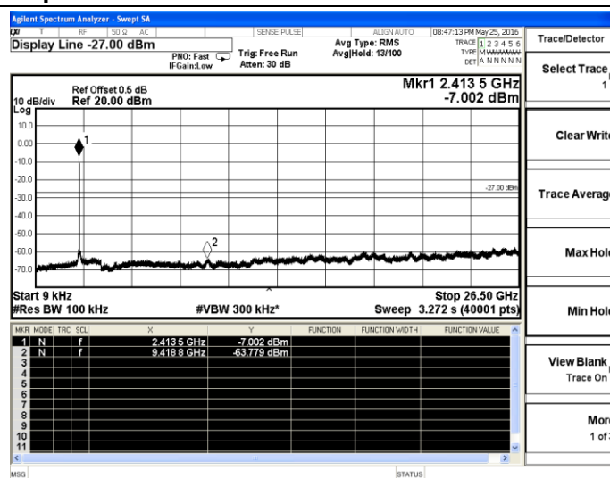
802.11g-Low channel
