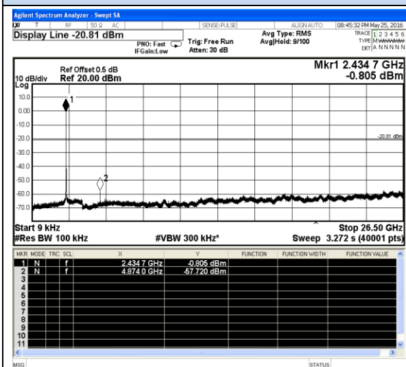
802.11b-Middle channel
