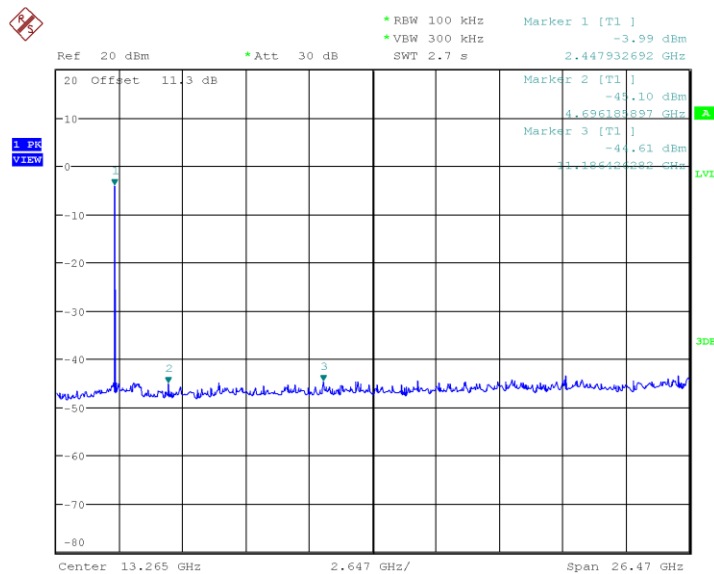
Plot 25. 2440MHz, 30MHz-26.5GHz Spurious
