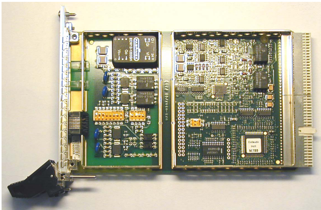
Figure 1 - ALB Board – internal side view of the ALB board
