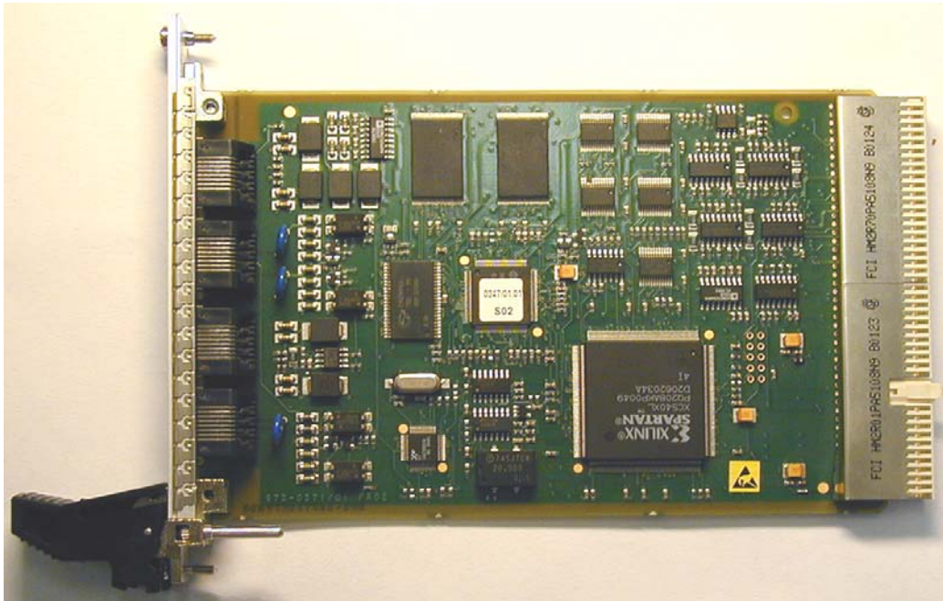
Figure 2 - IMC Board – side view of the IMC board
