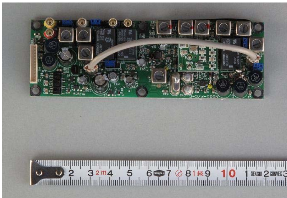
Picture 10 NT-2000 F/V Converter PCB
