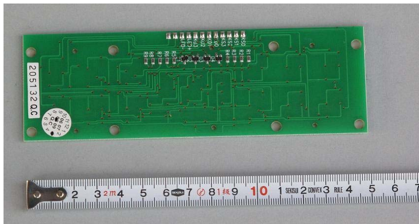
Picture 12 NT-2000 Keyboard PCB component side view
