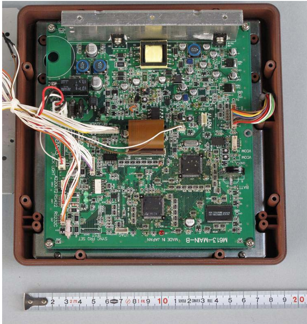
Picture 3 Main PCB including CPU, LCD and power supply circuit
