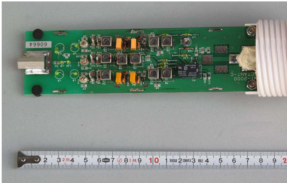
Picture 6 NT-1800 Active antenna PCB NT-2000 ACTANT-C
