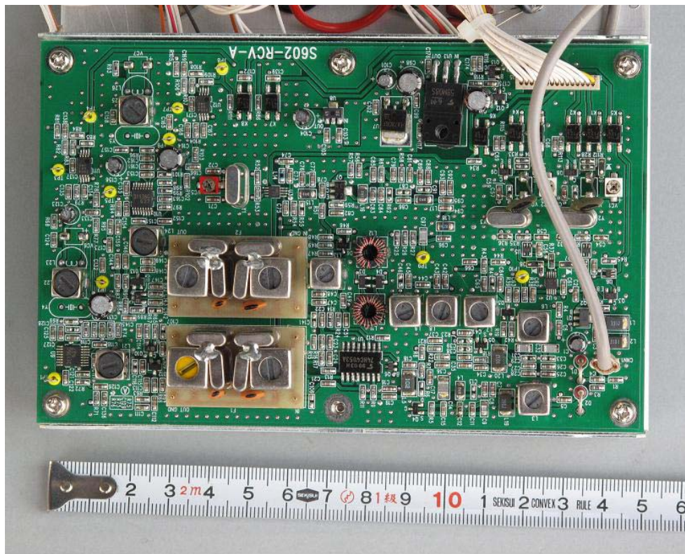
Picture 4 NT-1800 Receiver PCB S602-RCV-A
