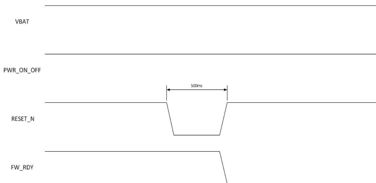
FIGURE 2 - POWER OFF SEQUENCE
