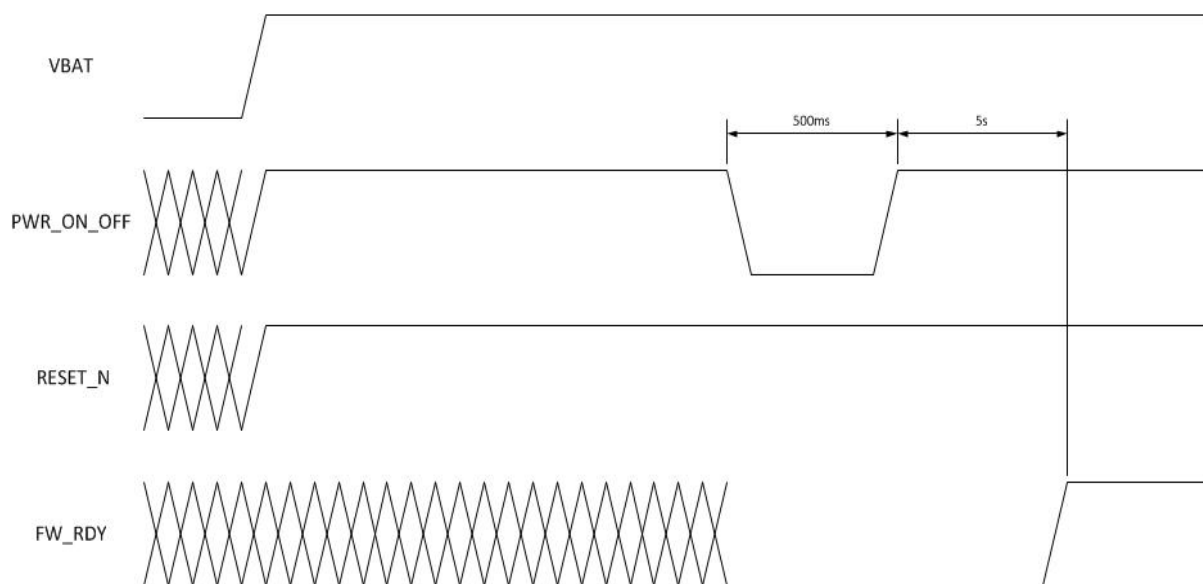
FIGURE 1 - POWER ON SEQUENCE
