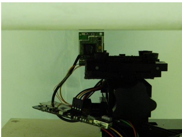
Top Side of the DUT with Phantom 0.2 cm Gap
