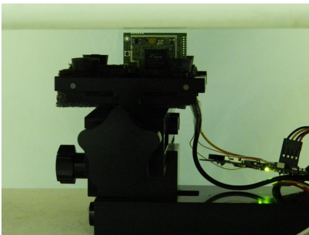
Right Side of the DUT with Phantom 0.2 cm Gap
