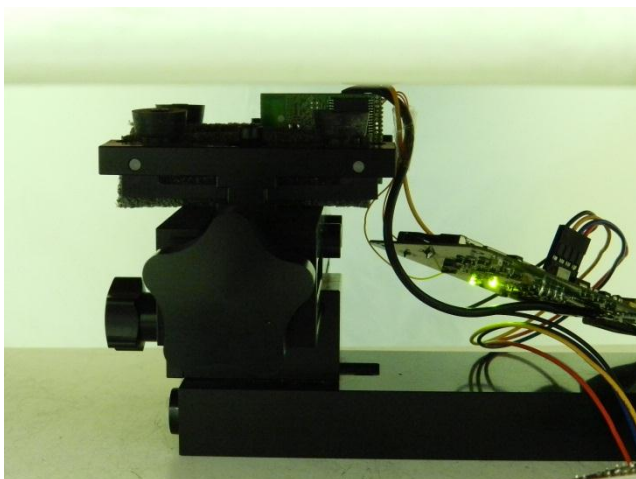
Left Side of the DUT with Phantom 0.2 cm Gap
