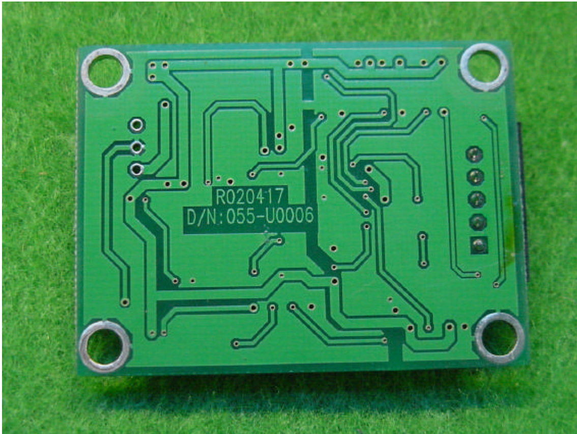
<Rear Photo of Touch panel Board>
