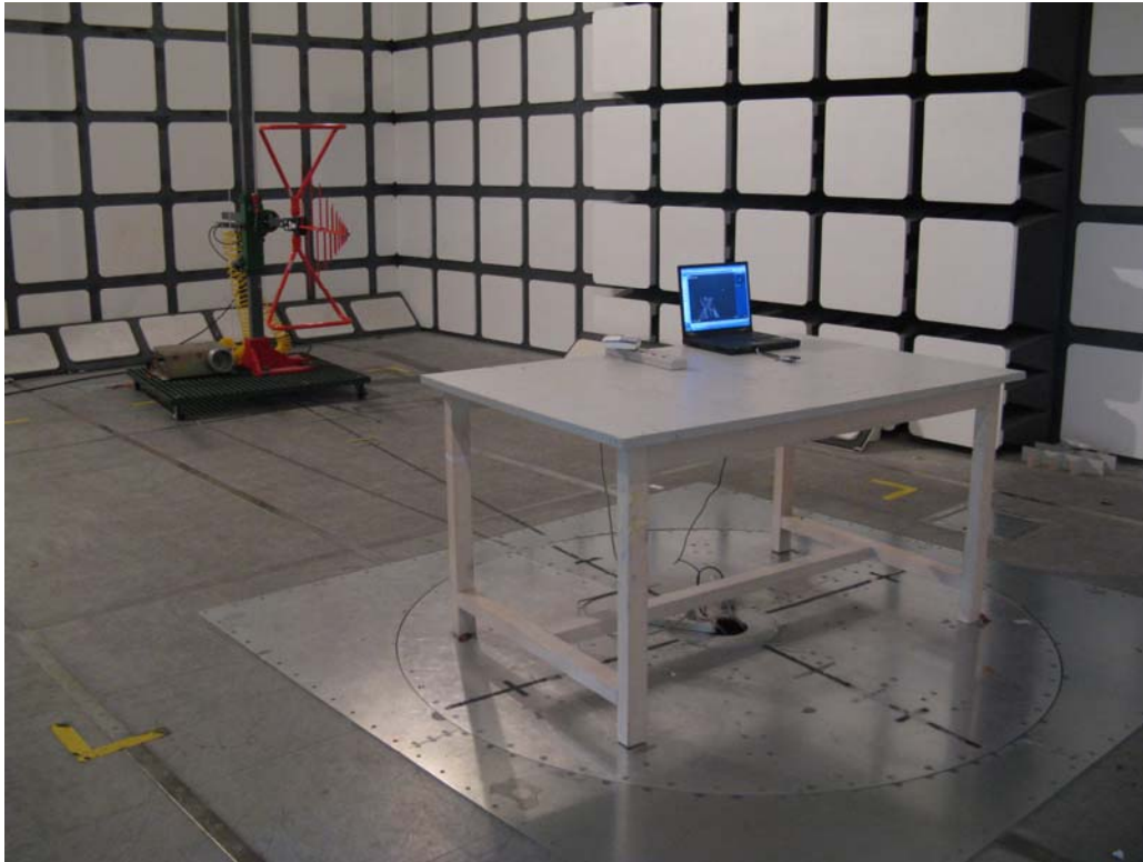
Radiated Emissions - Rear View (Below 1G)
