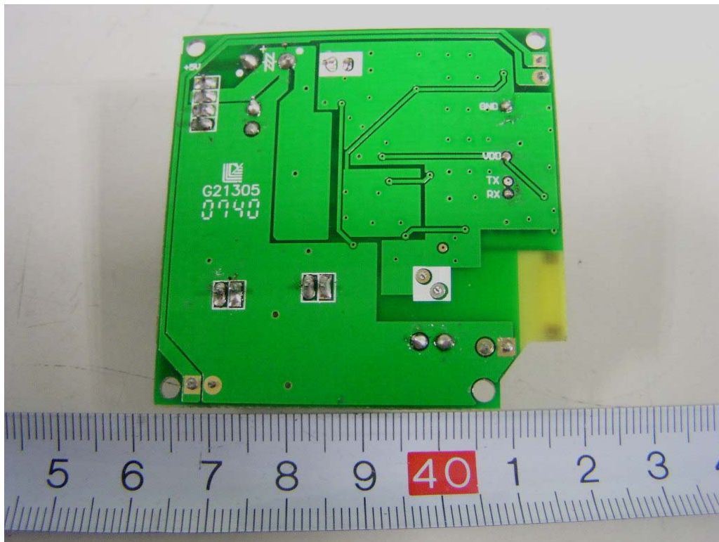
EUT (Red Color) –Main Board Bottom Components View
