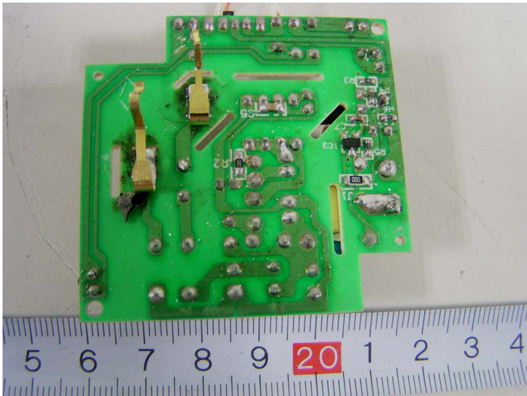
EUT (Red Color) –Power Board Bottom Components View (2)
