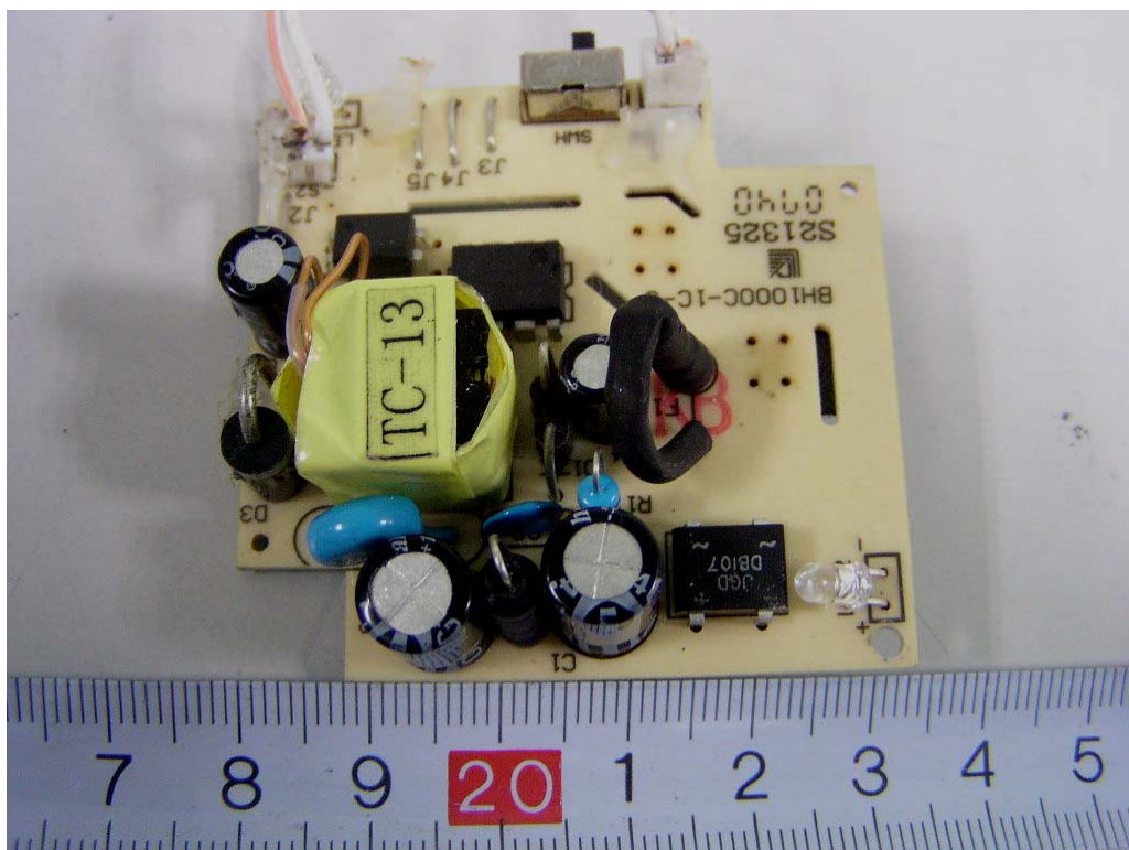
EUT (Red Color) –Power Board Top Components View
