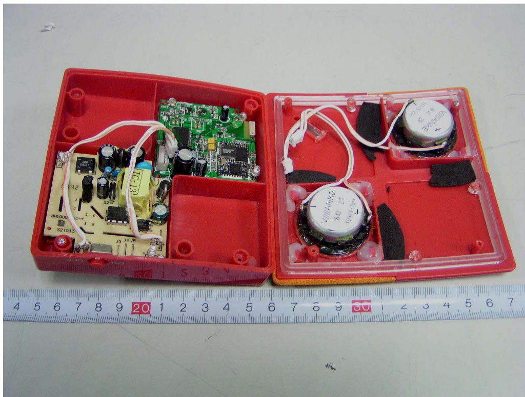
EUT (Red Color) –Uncovered View
