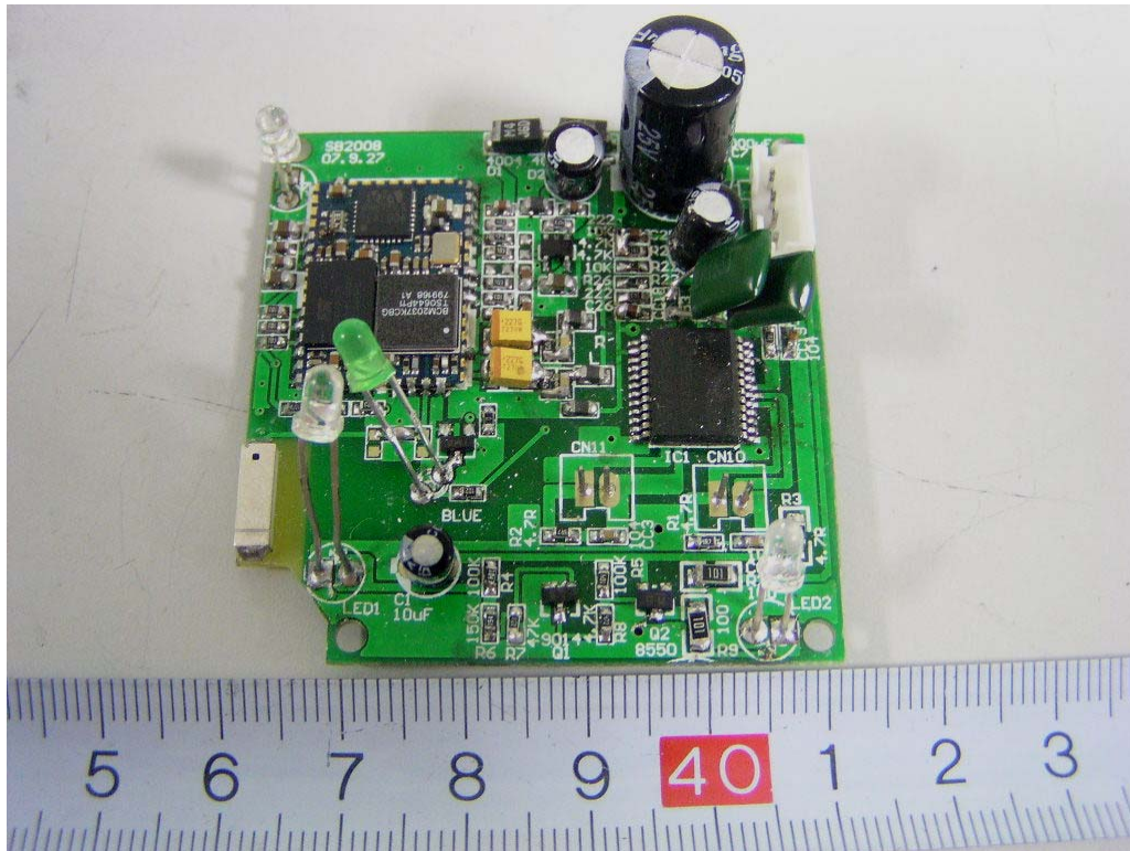
EUT (White Color) –Main Board Top Components View
