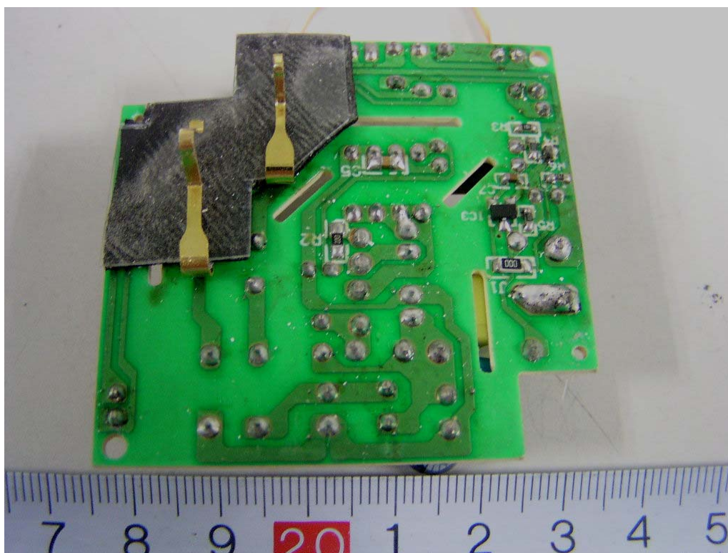
EUT (White Color) –Power Board Bottom Components View (1)
