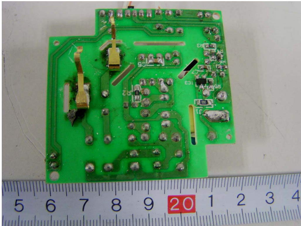
EUT (Black Color) –Power Board Bottom Components View (2)
