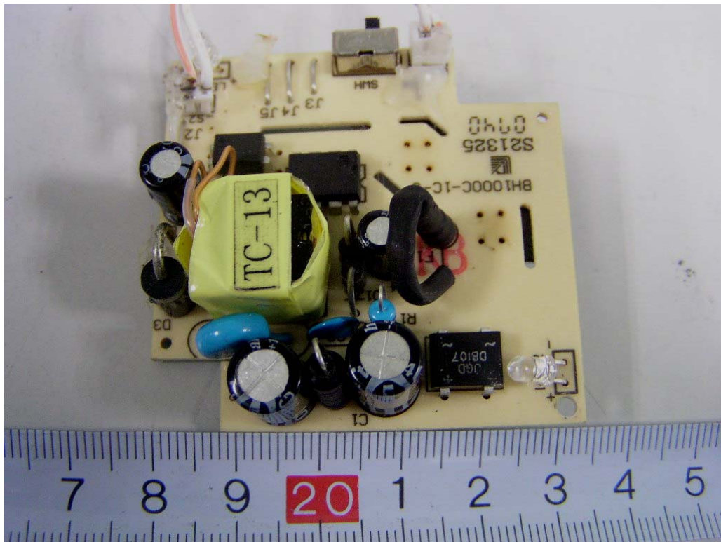
EUT (Black Color) –Power Board Top Components View
