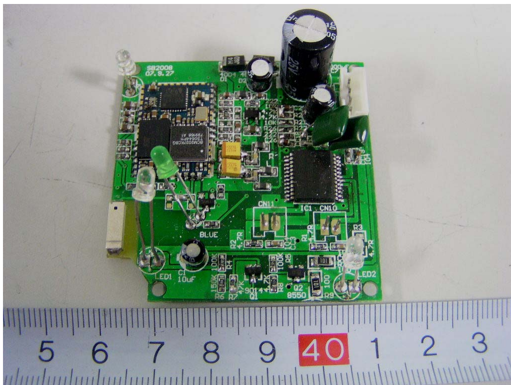
EUT (Red Color) –Main Board Top Components View
