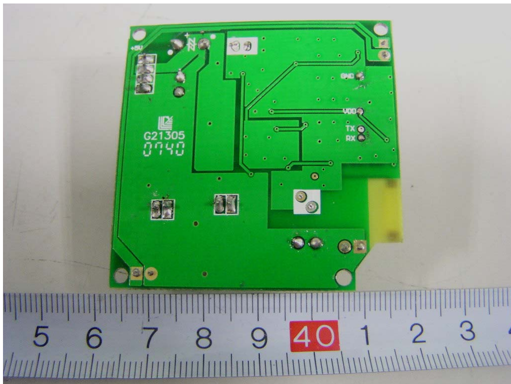
EUT (White Color) –Main Board Bottom Components View
