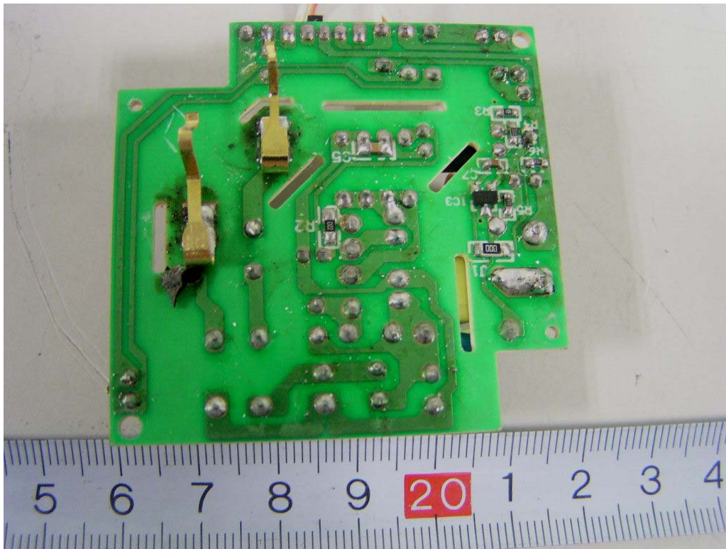
EUT (White Color) –Power Board Bottom Components View (2)
