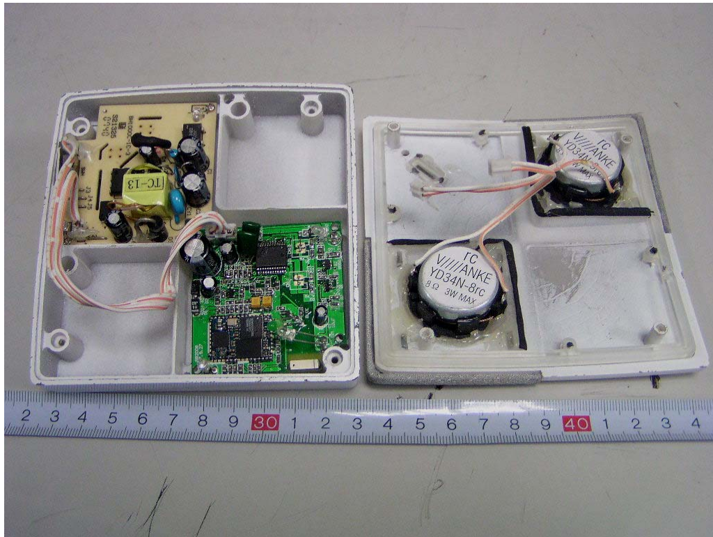
EUT (White Color) –Uncovered View
