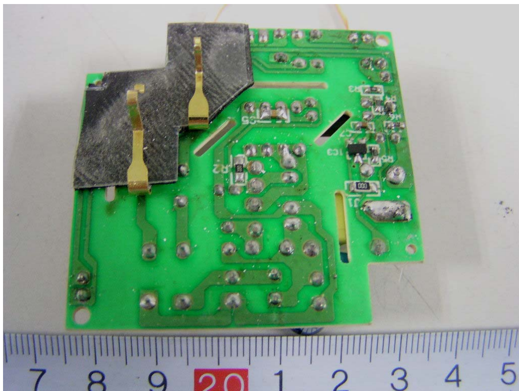
EUT (Black Color) –Power Board Bottom Components View (1)
