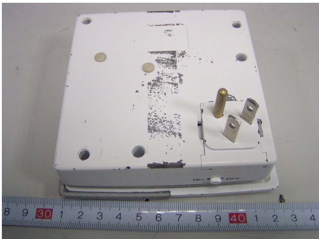
EUT (White Color) – Bottom View
