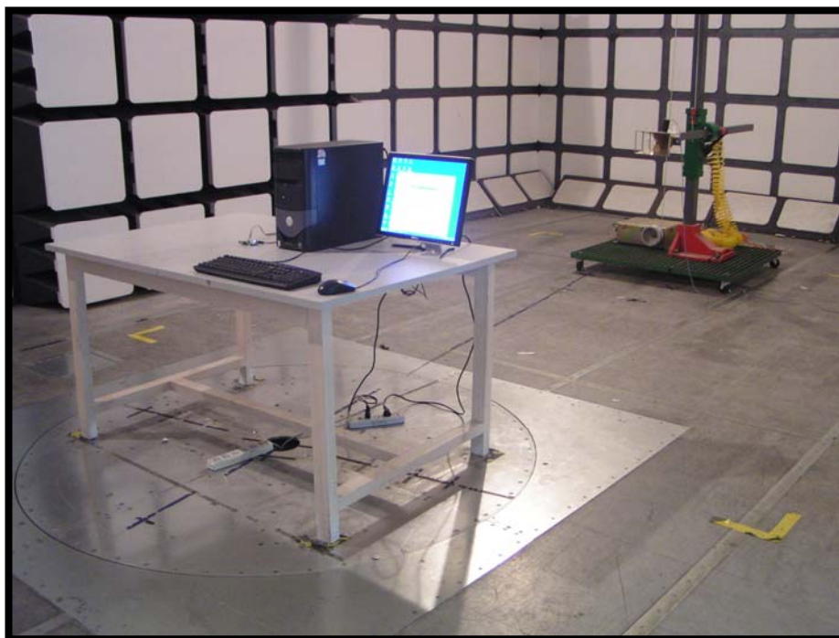
1 GHz-25GHz: Radiated Emission - Front View
