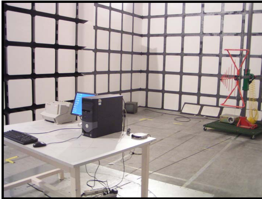
Charging mode: Radiated Emission - Front View
