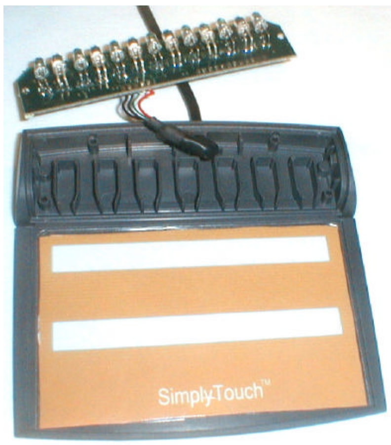
Internal view, PCB removed
