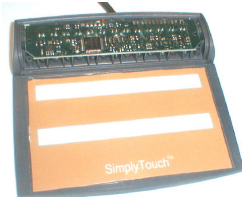
Internal view, Fences removed
