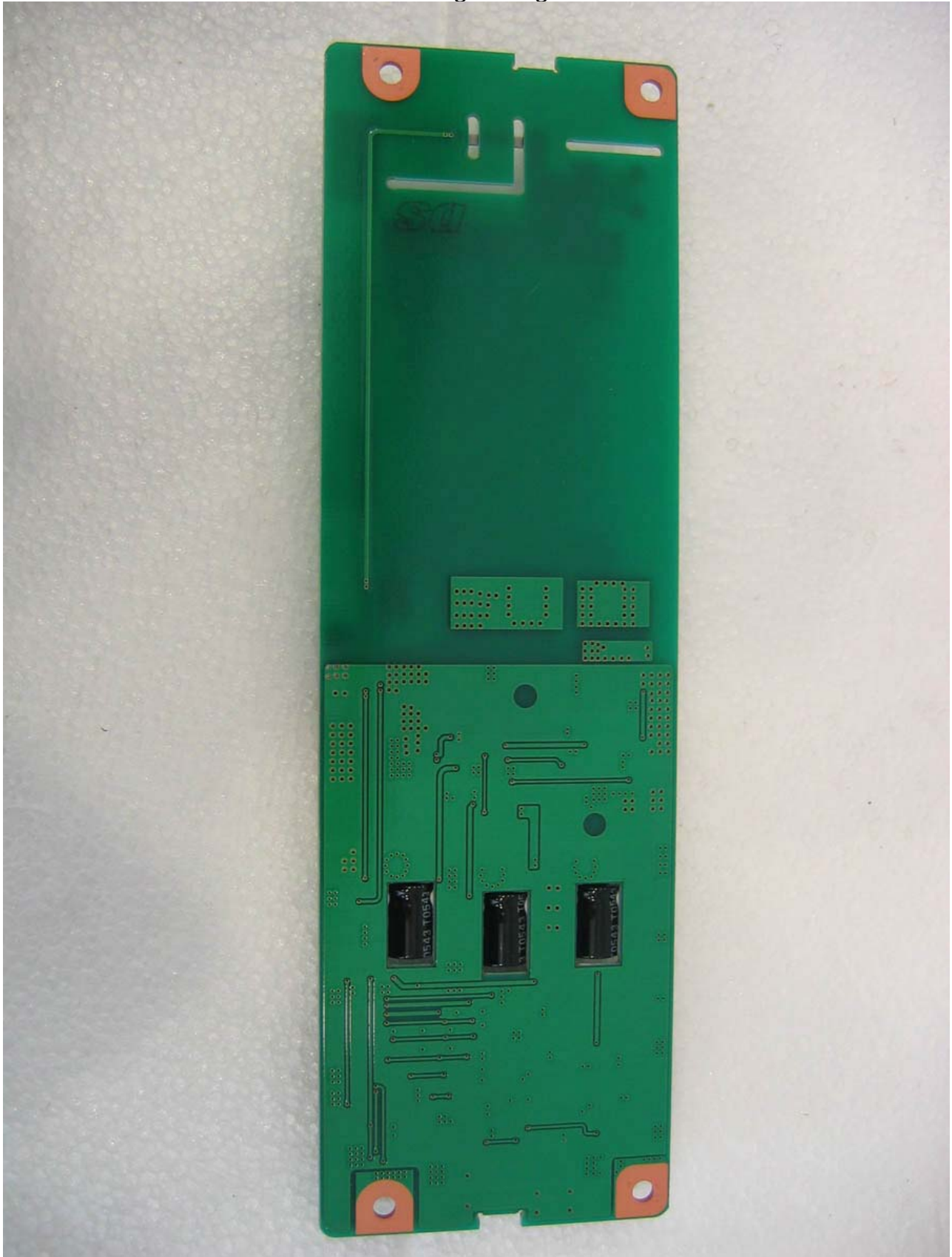
Bottom of high voltage board
