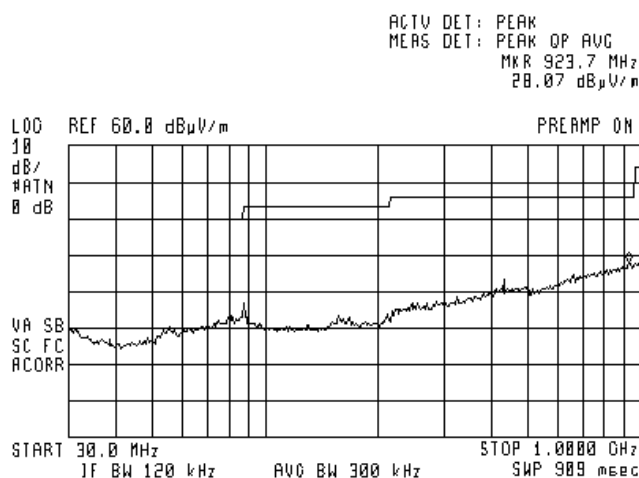
Plot 7.1.5 Radiated emission measurements from 30 to 1000 MHz
