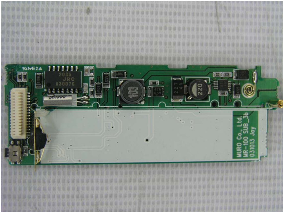
Sub board
