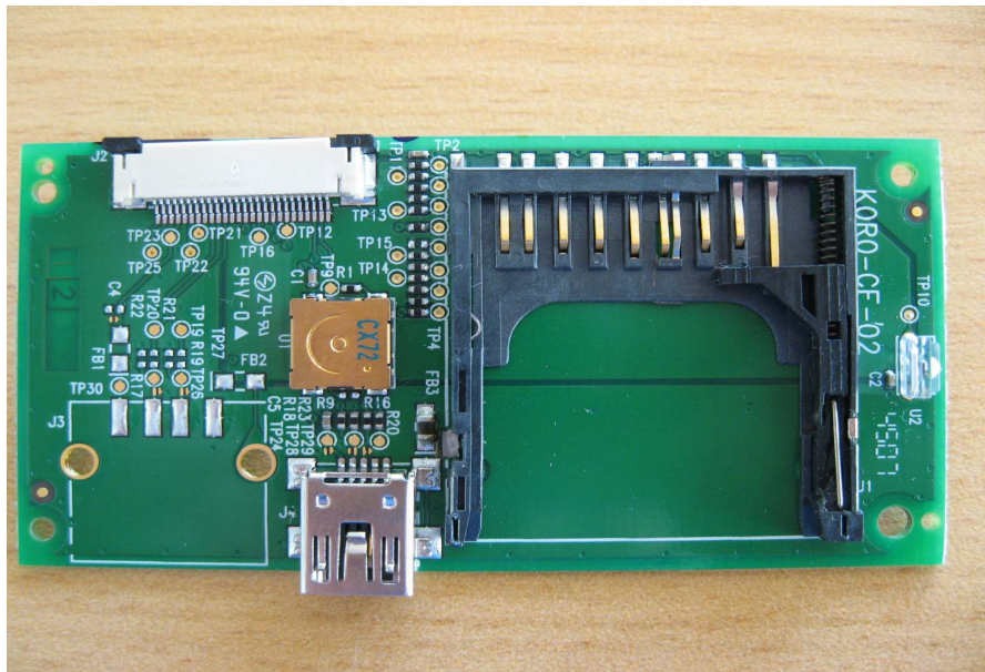
Daughter Board,Top with ( SD card connector )
