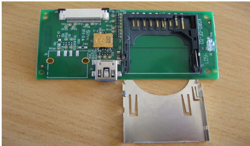
Daughter Board,Top with ( SD card connector )
