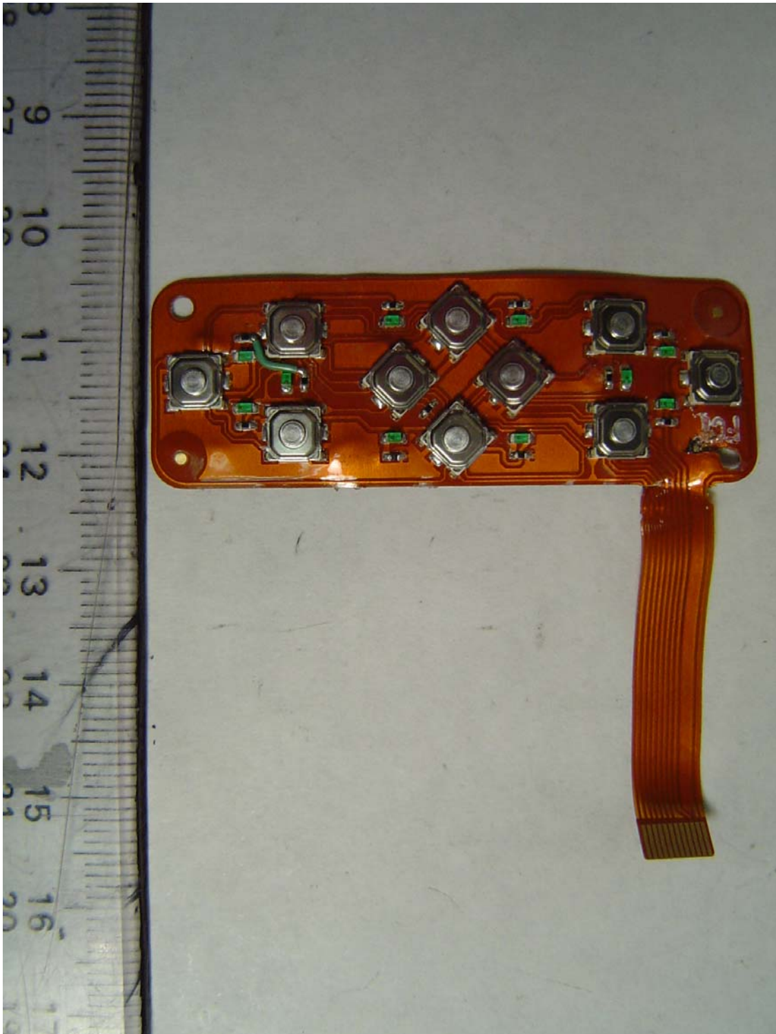
EUT Keypad Flexible Circuit – Front View
