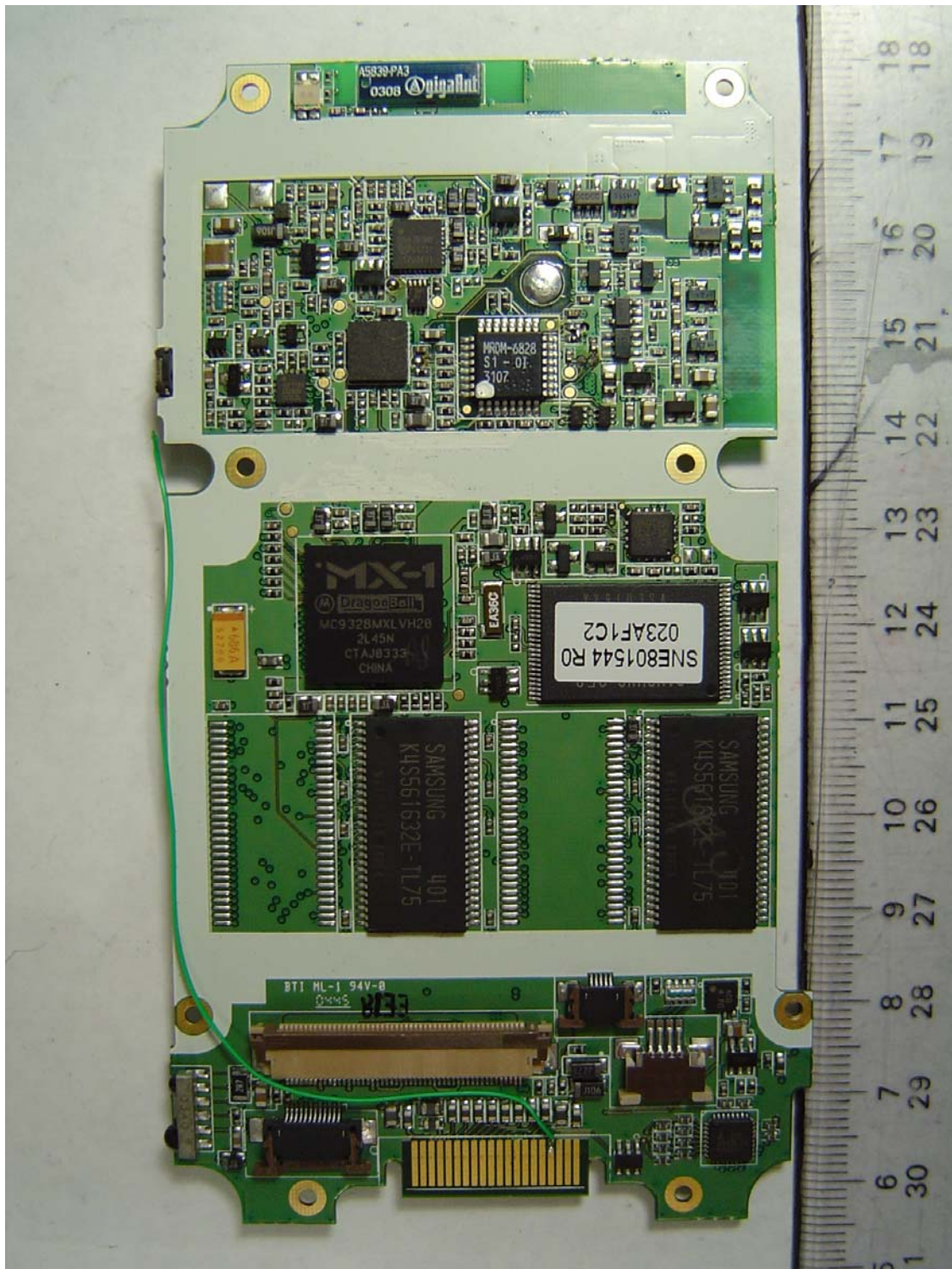
EUT Main PCB Component View
