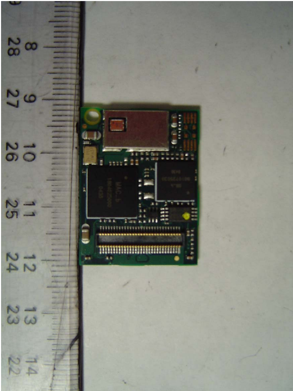
EUT RF Module Overall Trace View
