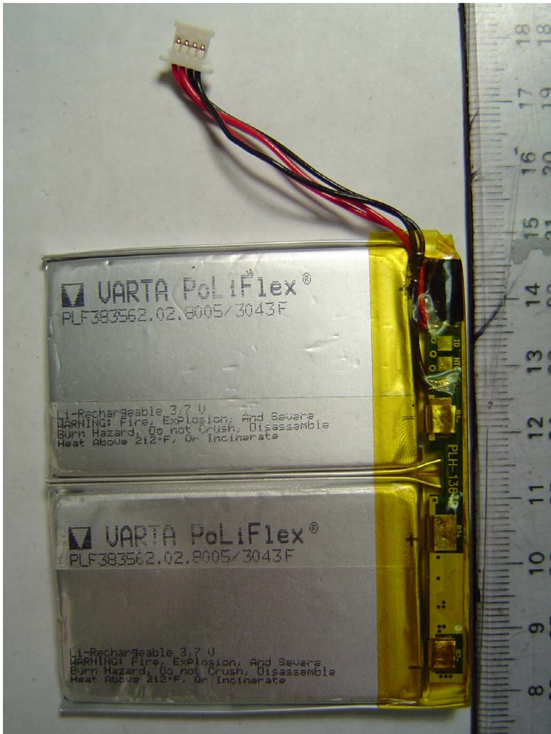
EUT Battery Front View
