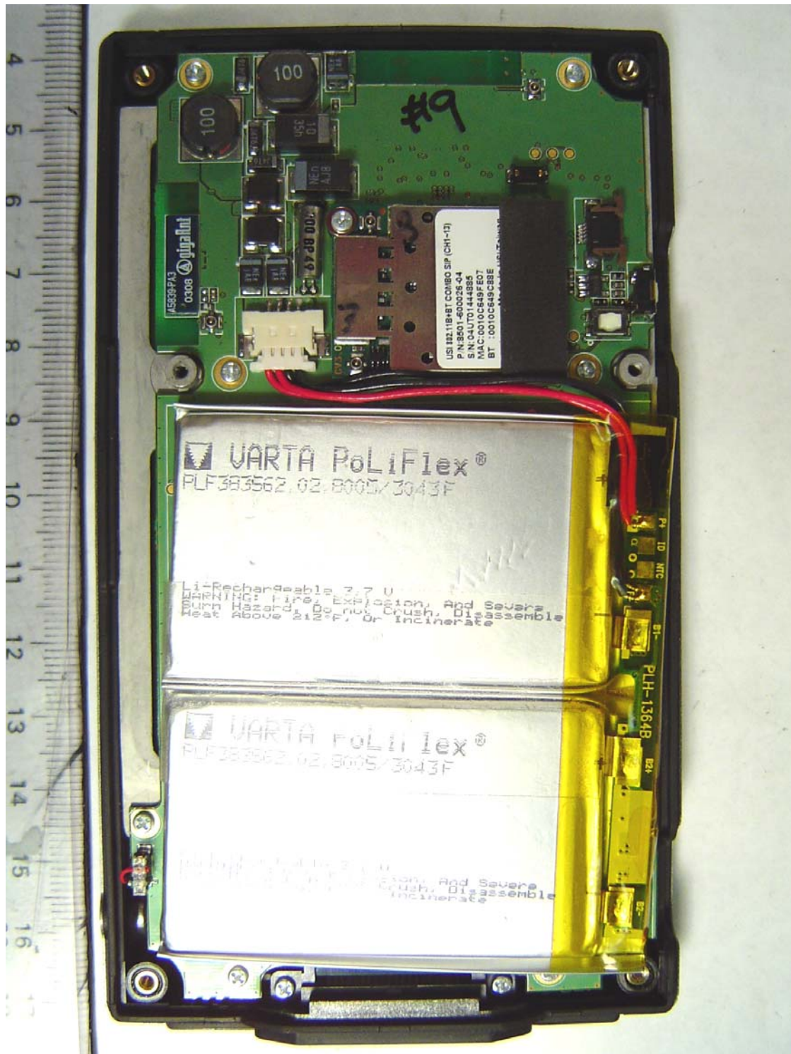
EUT Rear View (Rear Cover Removed)
