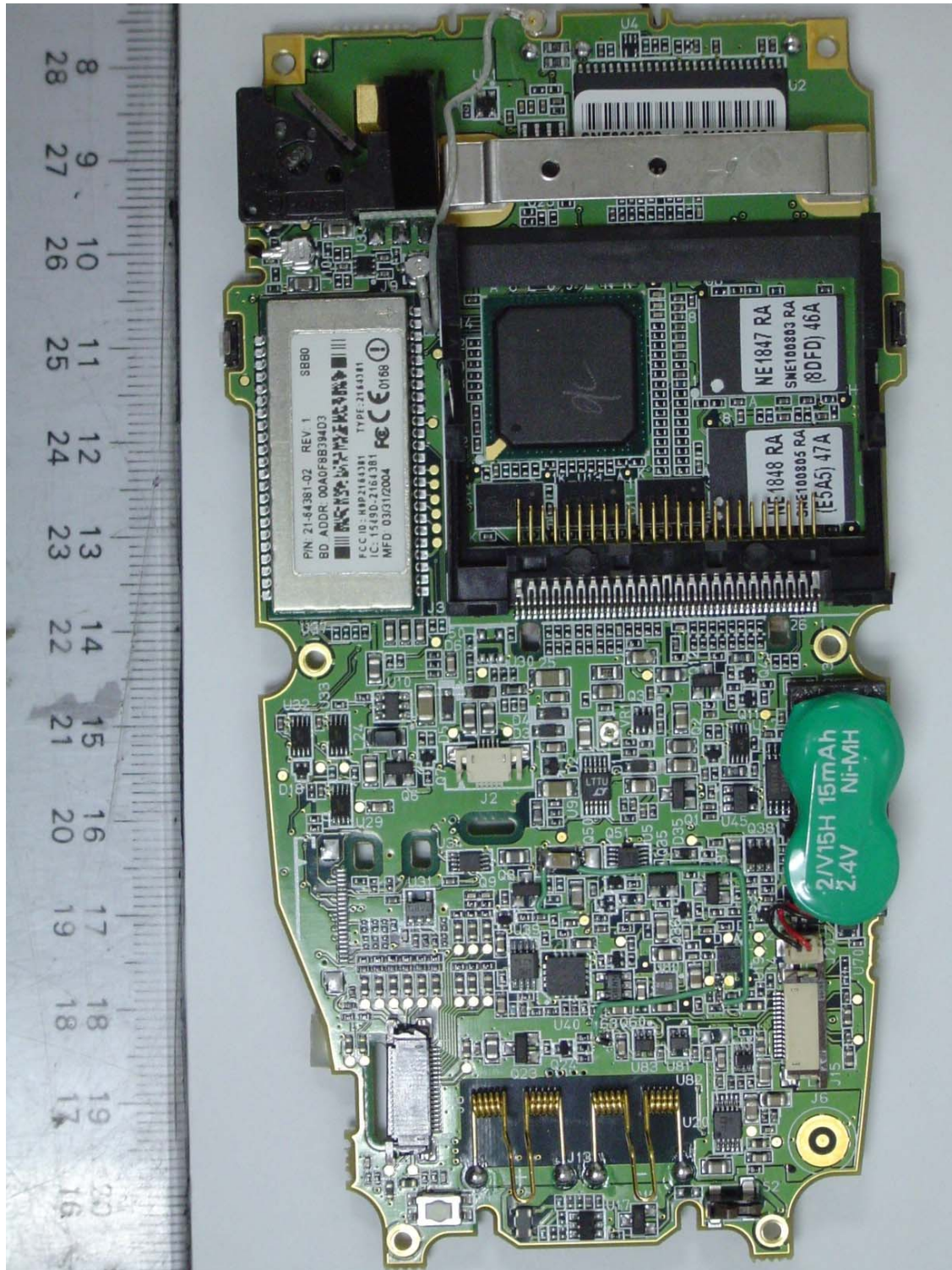
EUT Main Board PCB – Top View
