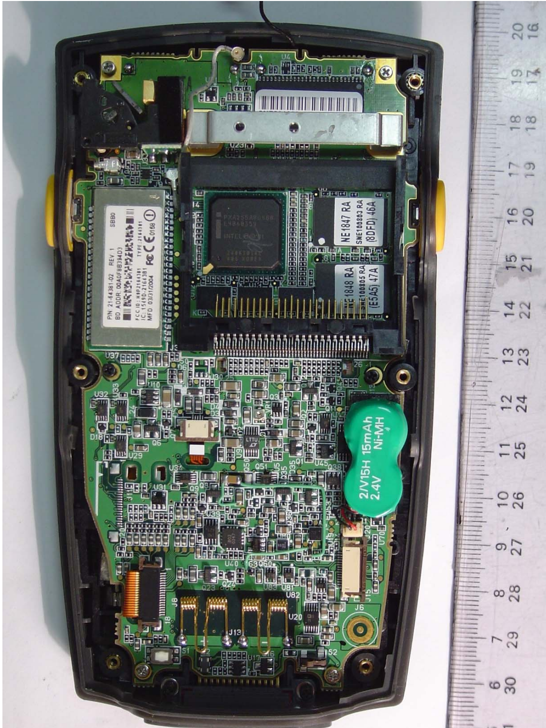
EUT Internal View (RF Module Removed)
