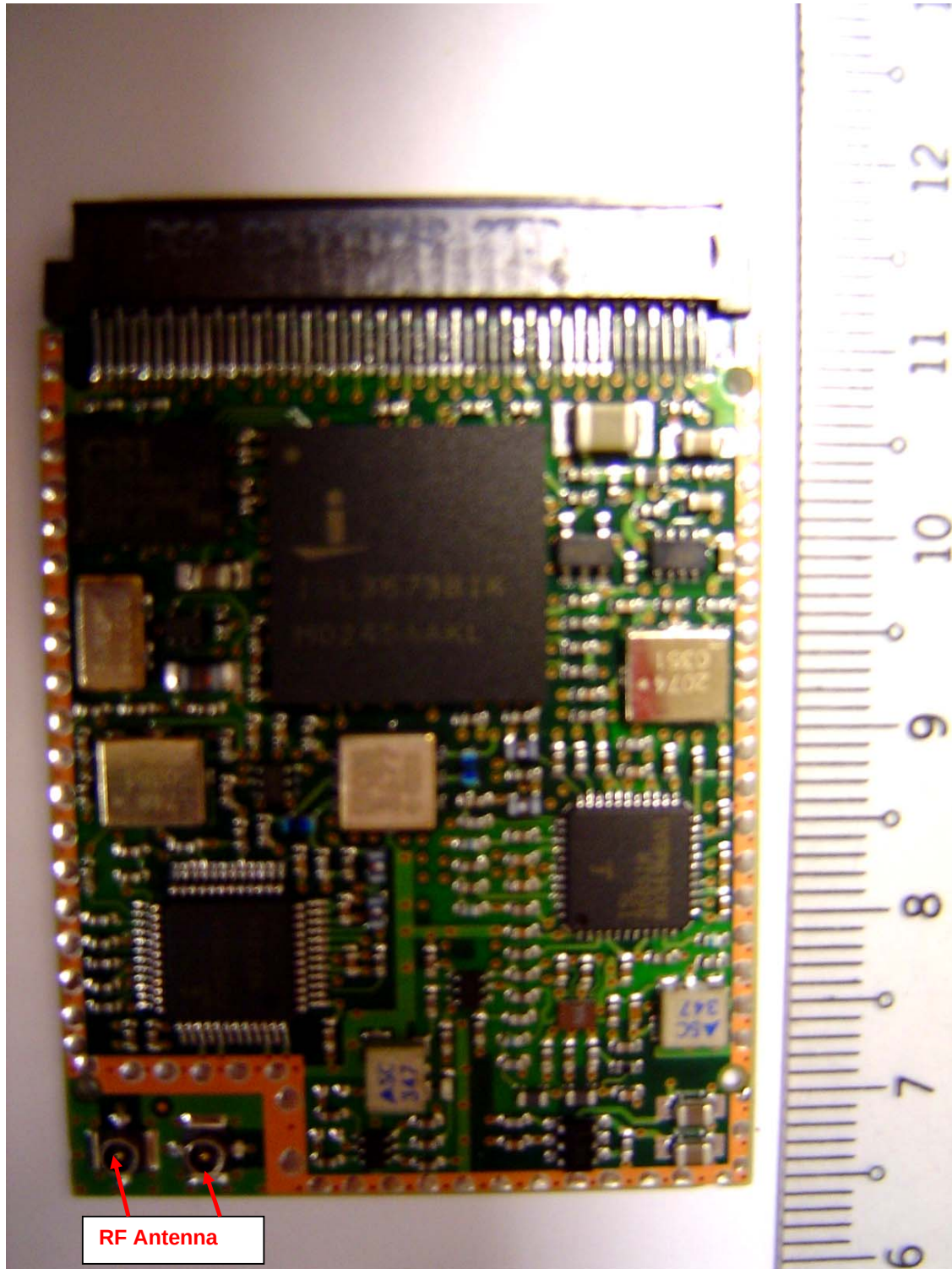
EUT RF Module – Top View
