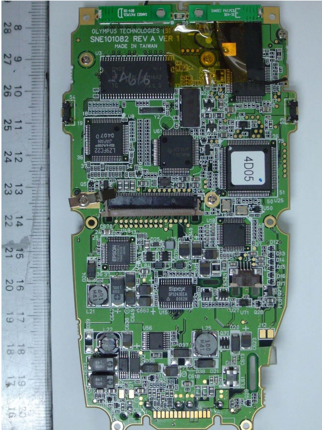
EUT Main Board PCB – Bottom View
