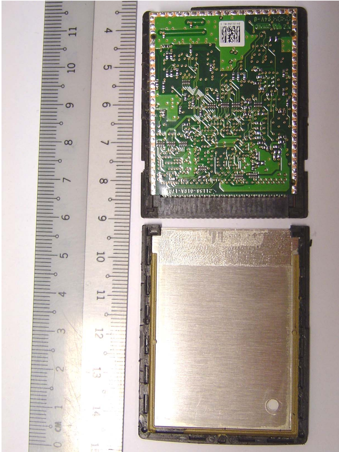
EUT RF Module Overall Internal View
