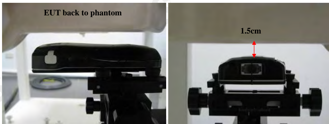
Fig.3 Testing body-worn SAR by separating 1.5cm between the back of the EUT
