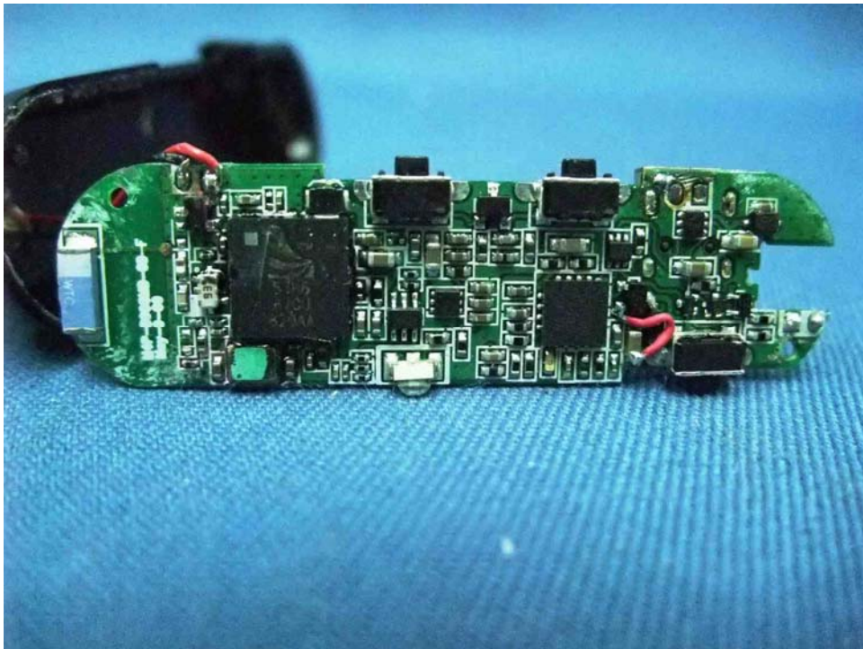
Bluetooth Headset Main PCB comp side
