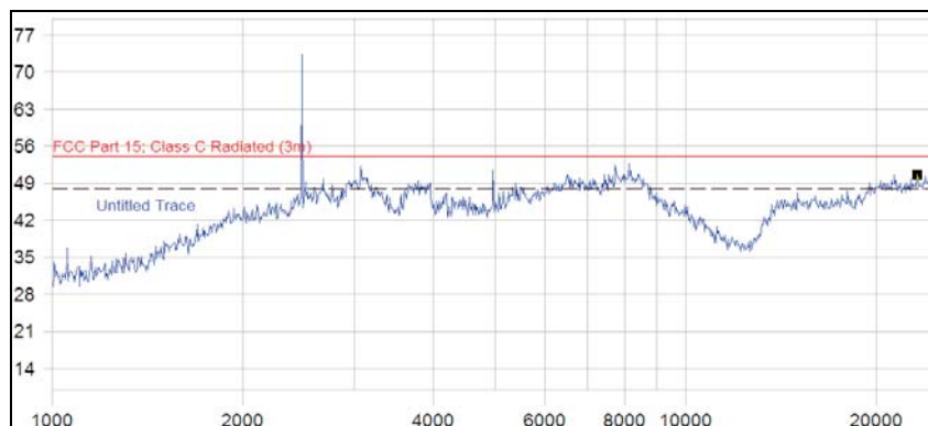
(Plot C.5: Antenna Vertical, 1GHz to 25GHz)
