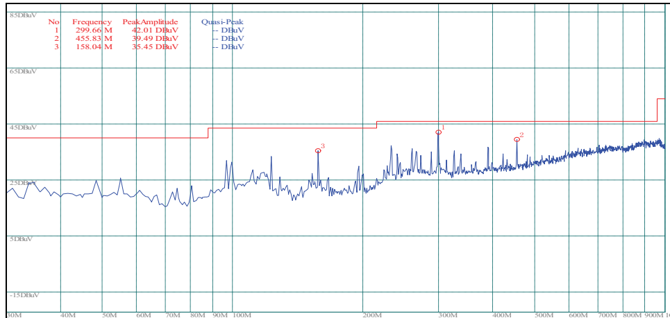
(Plot A4: Antenna Vertical, 30MHz to 1GHz)
