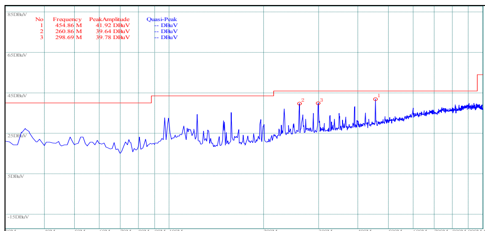
(Plot B4: Antenna Vertical, 30MHz to 1GHz)
