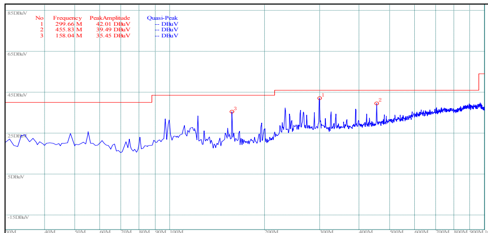
(Plot A4: Antenna Vertical, 30MHz to 1GHz)
