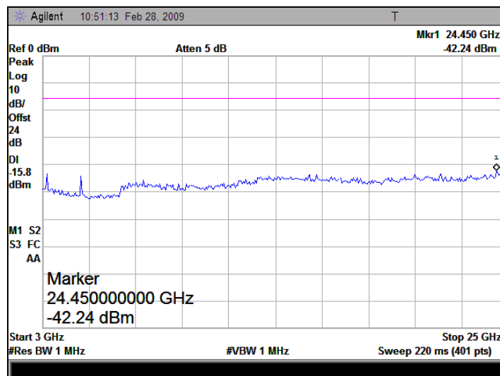
(Plot A.2: Channel = 0, 3GHz to 25GHz)
