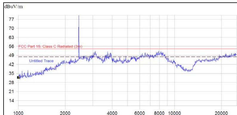
(Plot B.3: Antenna Horizontal, 1GHz to 25GHz)
