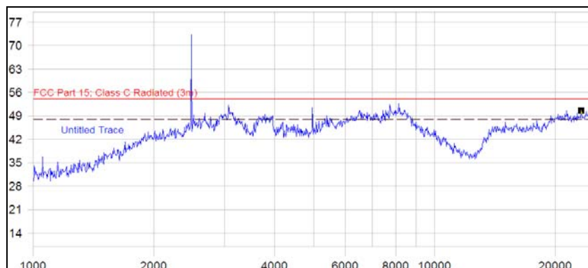
(Plot C.5: Antenna Vertical, 1GHz to 25GHz)
