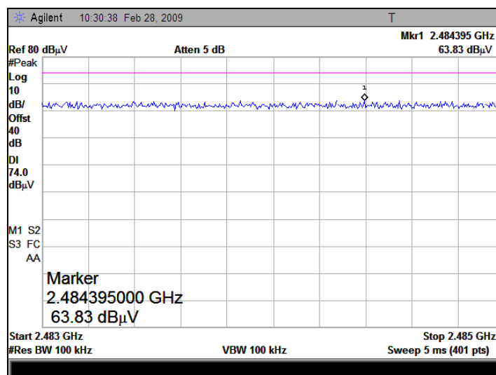
(Plot B1: Channel = 78 PEAK)
