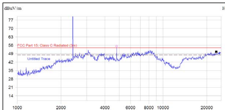
(Plot A.3: Antenna Horizontal, 1GHz to 25GHz)
