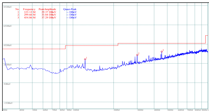
(Plot A.2: Antenna Horizontal, 30MHz to 1GHz)
