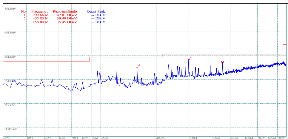
(Plot C.4: Antenna Vertical, 30MHz to 1GHz)
