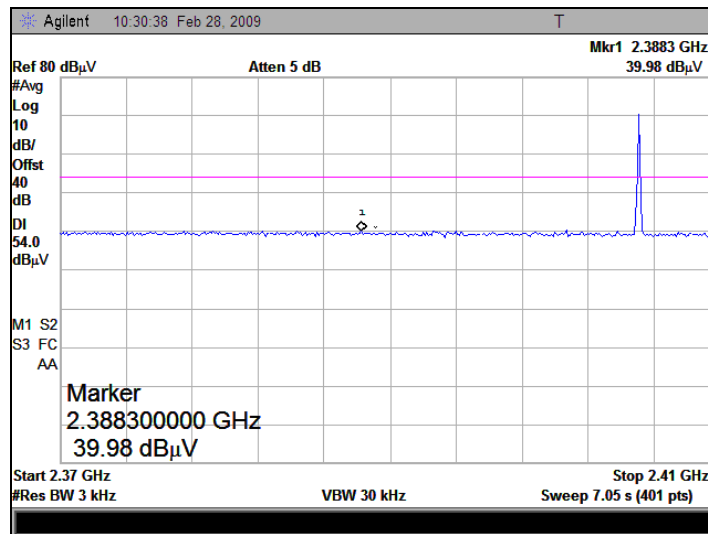
(Plot A2: Channel = 0 AVERAGE)
