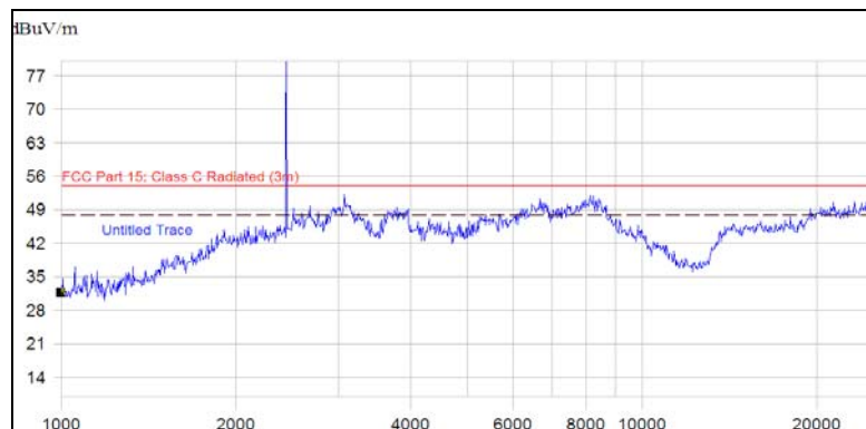
(Plot B5: Antenna Vertical, 1GHz to 25GHz)
