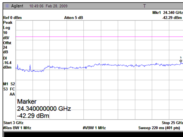
(Plot B.2: Channel = 39, 3GHz to 25GHz)
