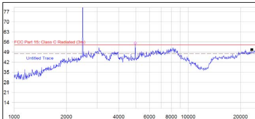
(Plot C.3: Antenna Horizontal, 1GHz to 25GHz)
