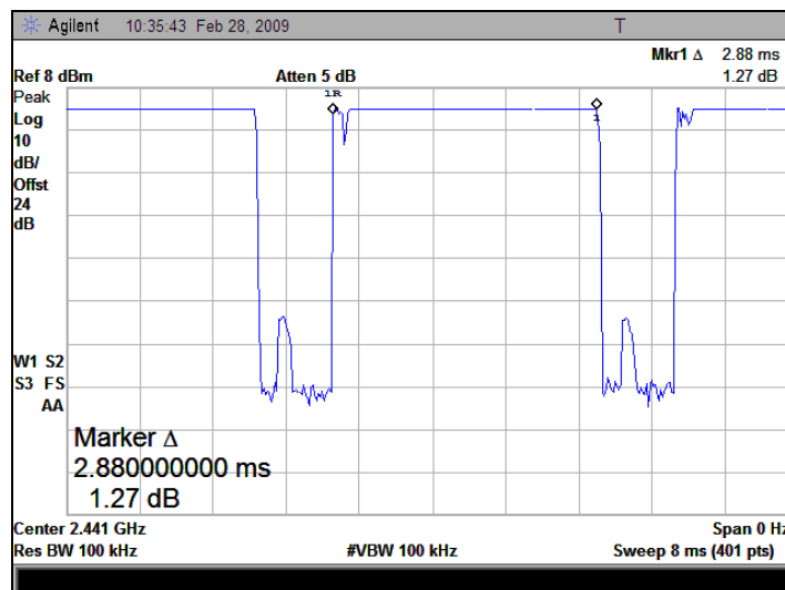
(Plot B: Channel = 2441)
