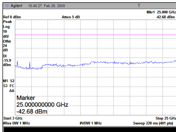
(Plot C.2: Channel = 78, 3GHz to 25GHz)
