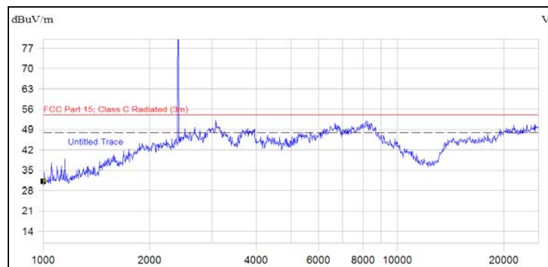
(Plot A.5: Antenna Vertical, 1GHz to 25GHz)
