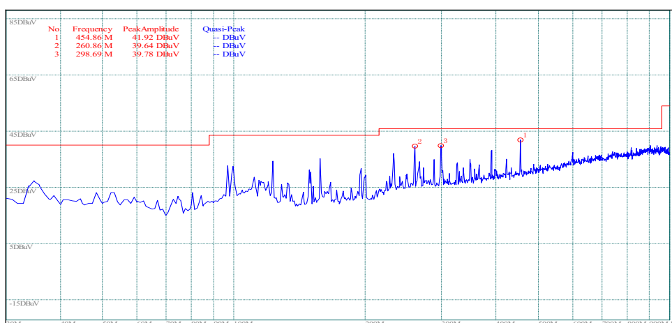
(Plot B4: Antenna Vertical, 30MHz to 1GHz)
