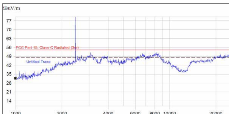
(Plot B5: Antenna Vertical, 1GHz to 25GHz)
