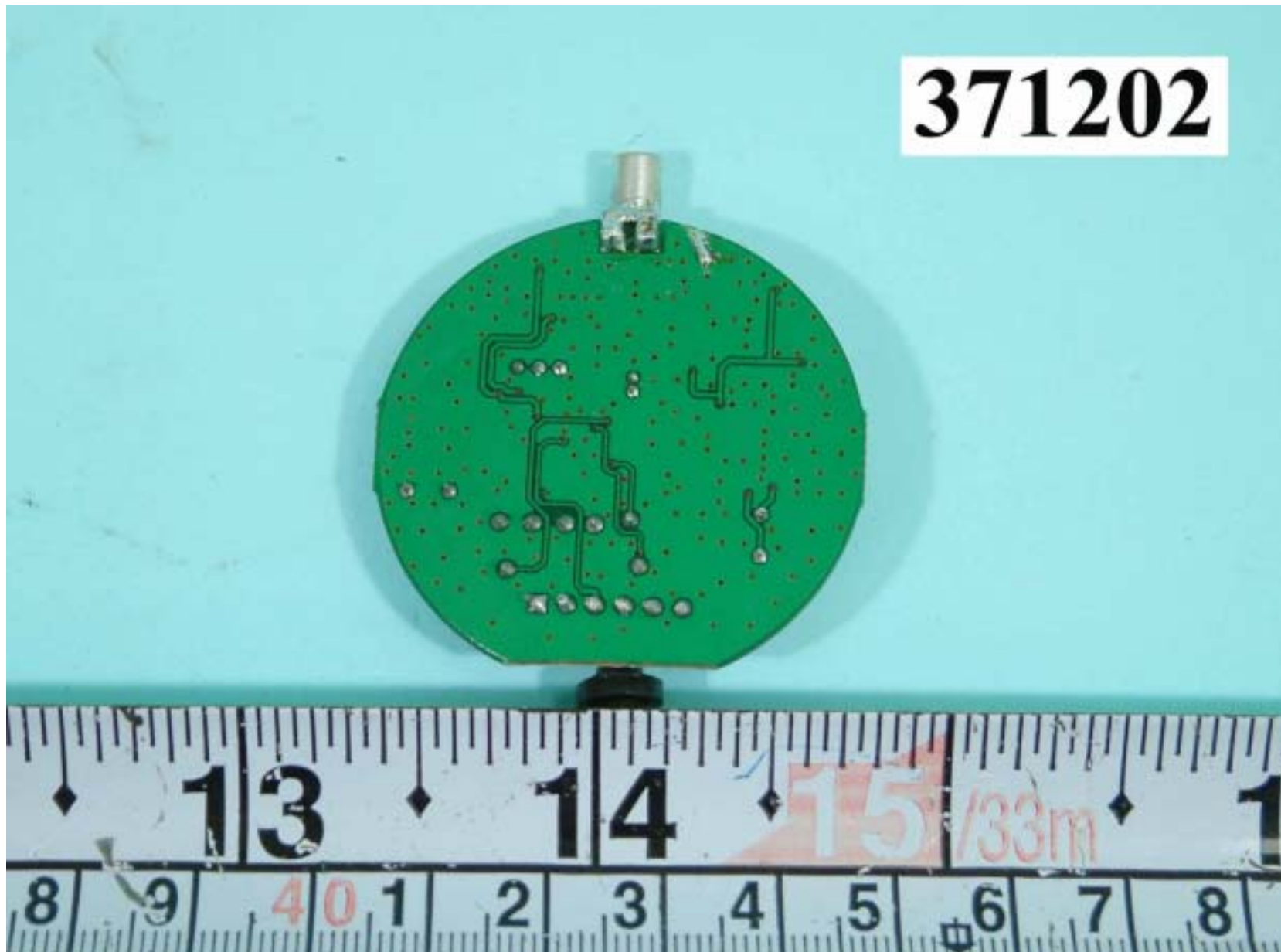
REAR SIDE OF MAIN BOARD OF TRANSCEIVER
