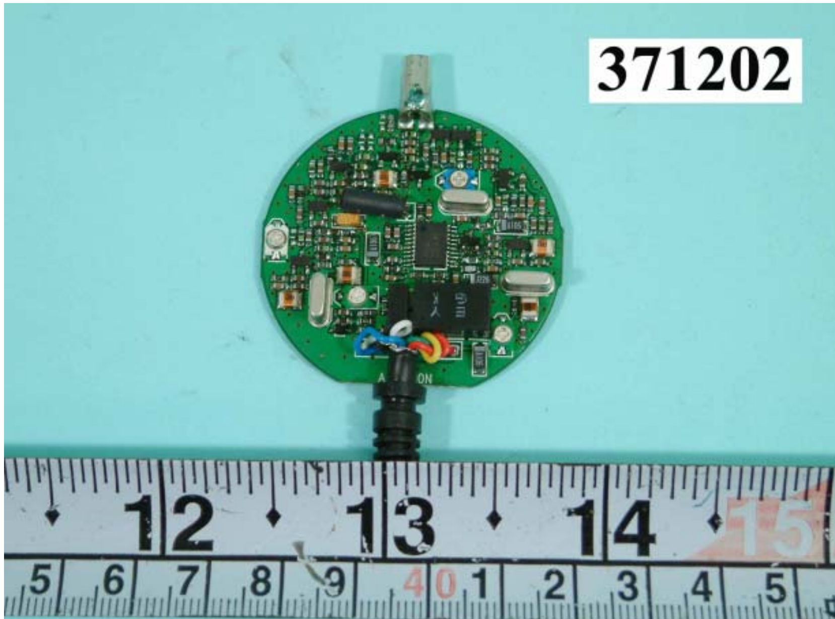
FRONT SIDE OF MAIN BOARD OF TRANSCEIVER
