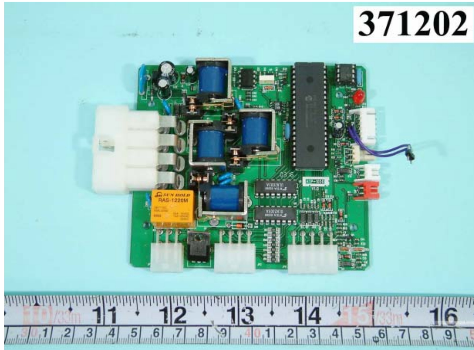
FRONT SIDE OF MAIN BOARD OF EUT
