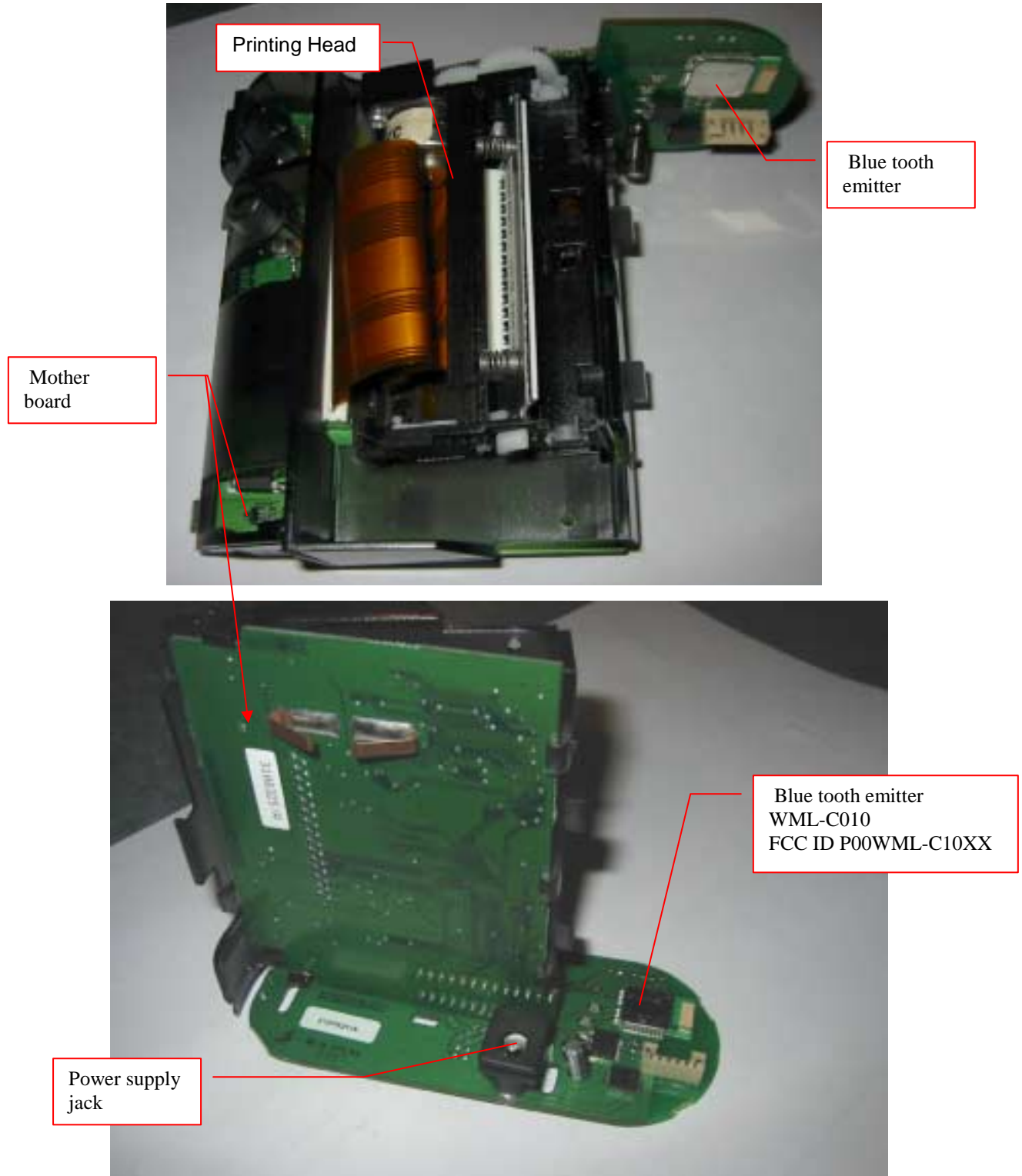
Figure 2: Cover removed (top and bottom Views)
