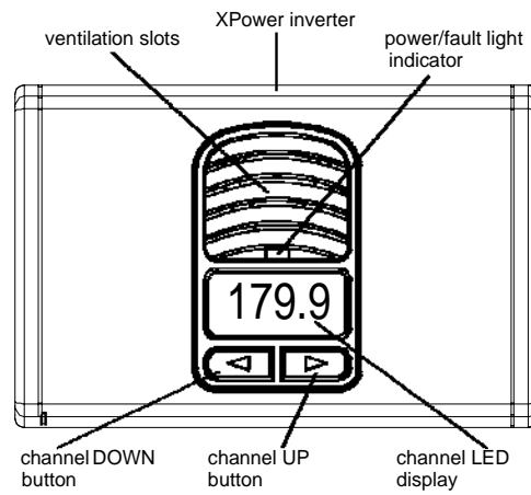
Figure 3 Channel Tuner
